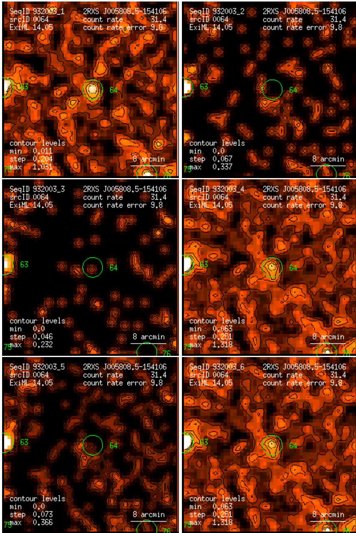
Figure 64: RASS 932003: detection 0064: band rate images, Gaussian filter: (1) PSPC channels 11 – 41, (2) 52 – 90, (3) 91 – 201, (4) 11 – 235, (5) 52 – 201, (6) 11 – 201. Broad band rates in counts/ks. Band rate contour levels in counts/ks/arcmin 2 .
