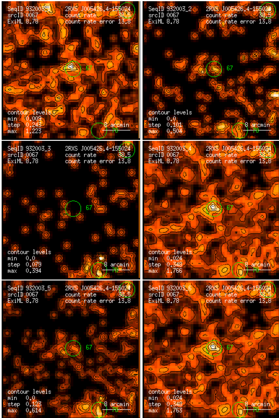
Figure 67: RASS 932003: detection 0067: band rate images, Gaussian filter: (1) PSPC channels 11 – 41, (2) 52 – 90, (3) 91 – 201, (4) 11 – 235, (5) 52 – 201, (6) 11 – 201. Broad band rates in counts/ks. Band rate contour levels in counts/ks/arcmin 2 .
