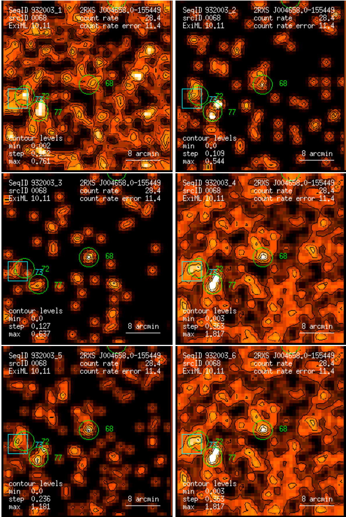
Figure 68: RASS 932003: detection 0068: band rate images, Gaussian filter: (1) PSPC channels 11 – 41, (2) 52 – 90, (3) 91 – 201, (4) 11 – 235, (5) 52 – 201, (6) 11 – 201. Broad band rates in counts/ks. Band rate contour levels in counts/ks/arcmin 2 .
