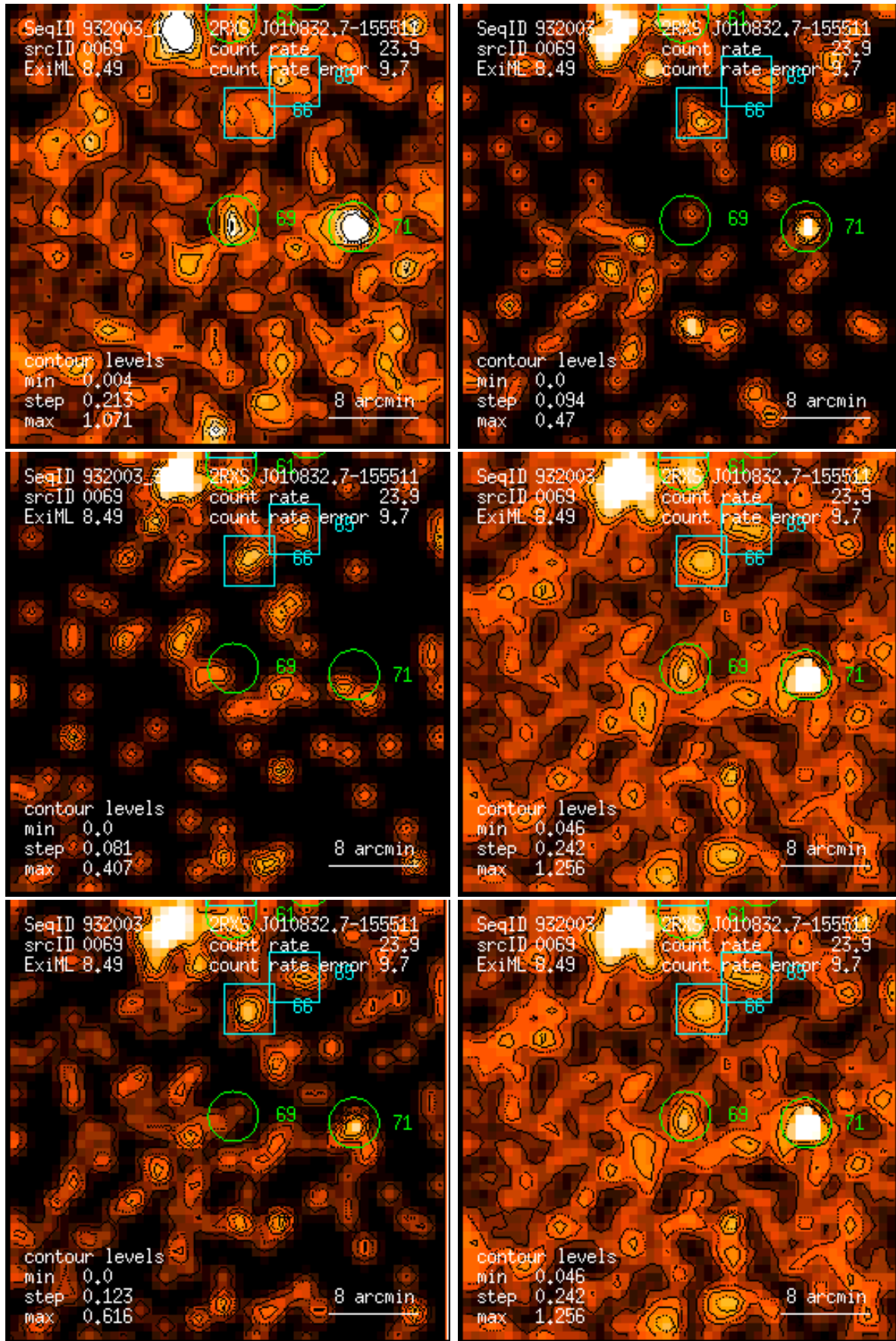
Figure 69: RASS 932003: detection 0069: band rate images, Gaussian filter: (1) PSPC channels 11 – 41, (2) 52 – 90, (3) 91 – 201, (4) 11 – 235, (5) 52 – 201, (6) 11 – 201. Broad band rates in counts/ks. Band rate contour levels in counts/ks/arcmin 2 .
