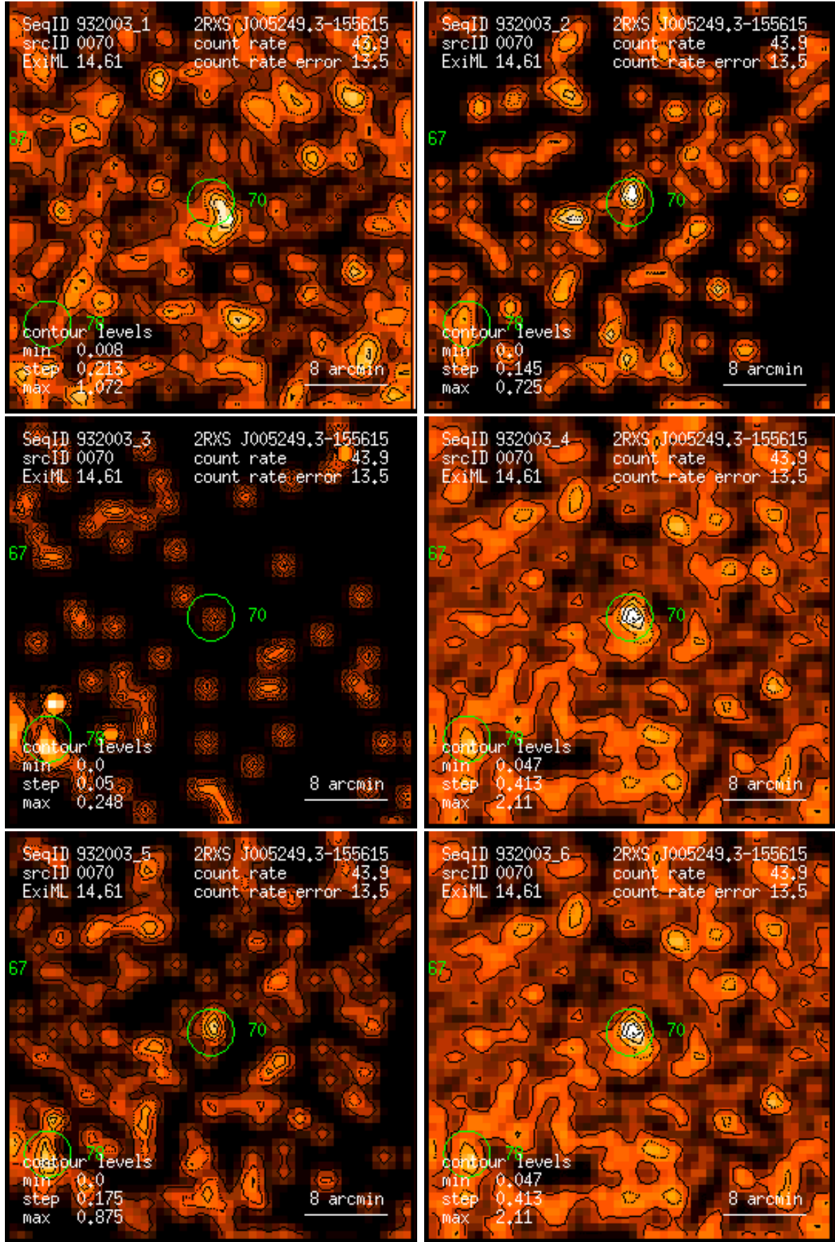
Figure 70: RASS 932003: detection 0070: band rate images, Gaussian filter: (1) PSPC channels 11 – 41, (2) 52 – 90, (3) 91 – 201, (4) 11 – 235, (5) 52 – 201, (6) 11 – 201. Broad band rates in counts/ks. Band rate contour levels in counts/ks/arcmin 2 .
