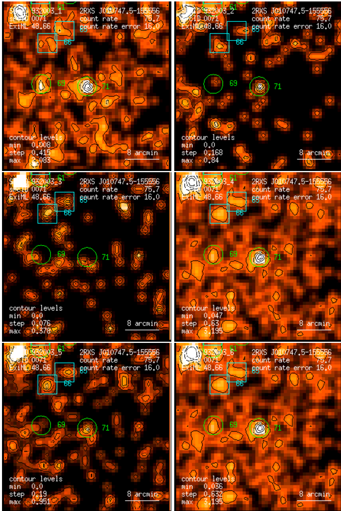
Figure 71: RASS 932003: detection 0071: band rate images, Gaussian filter: (1) PSPC channels 11 – 41, (2) 52 – 90, (3) 91 – 201, (4) 11 – 235, (5) 52 – 201, (6) 11 – 201. Broad band rates in counts/ks. Band rate contour levels in counts/ks/arcmin 2 .
