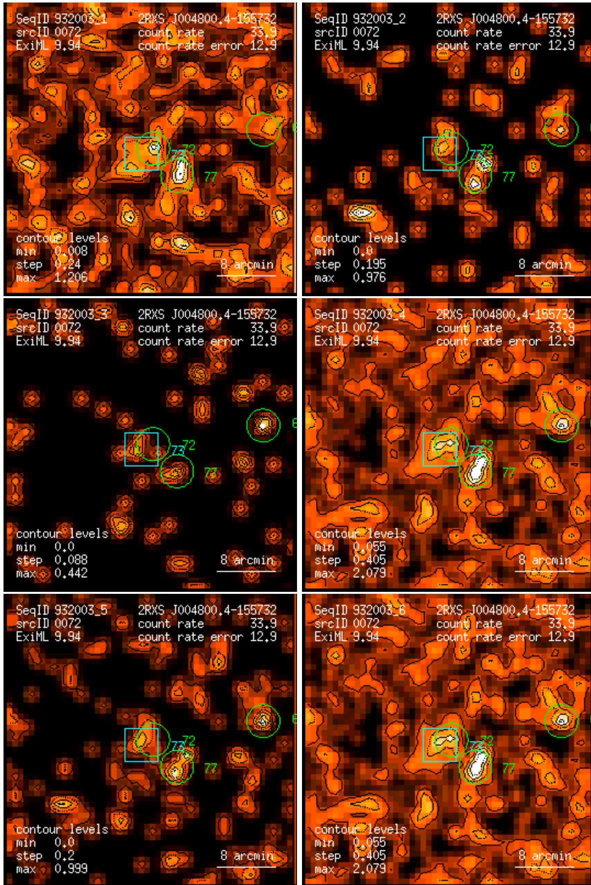
Figure 72: RASS 932003: detection 0072: band rate images, Gaussian filter: (1) PSPC channels 11 – 41, (2) 52 – 90, (3) 91 – 201, (4) 11 – 235, (5) 52 – 201, (6) 11 – 201. Broad band rates in counts/ks. Band rate contour levels in counts/ks/arcmin 2 .
