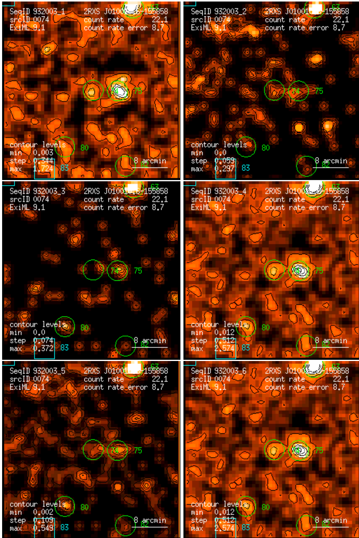
Figure 74: RASS 932003: detection 0074: band rate images, Gaussian filter: (1) PSPC channels 11 – 41, (2) 52 – 90, (3) 91 – 201, (4) 11 – 235, (5) 52 – 201, (6) 11 – 201. Broad band rates in counts/ks. Band rate contour levels in counts/ks/arcmin 2 .
