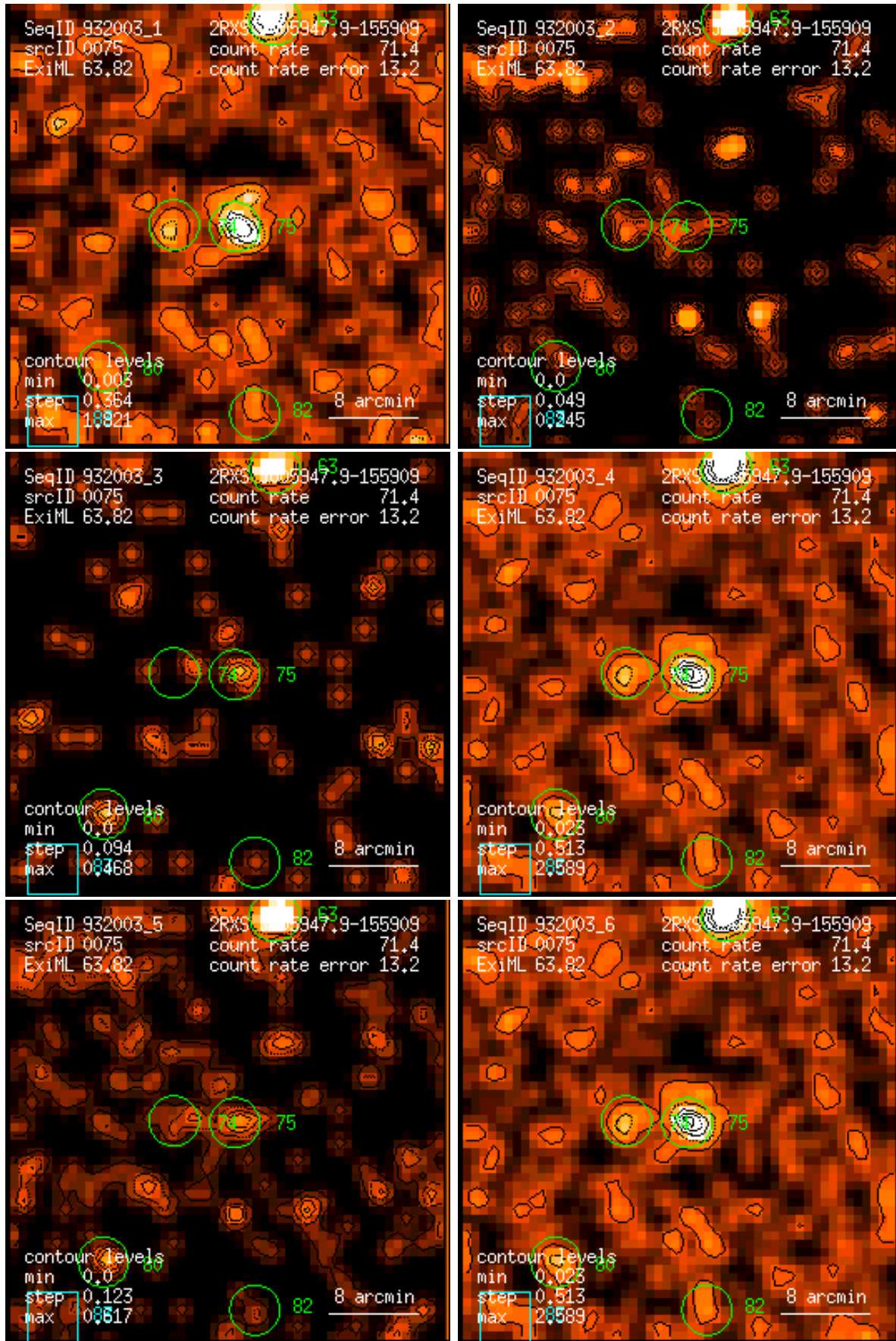
Figure 75: RASS 932003: detection 0075: band rate images, Gaussian filter: (1) PSPC channels 11 – 41, (2) 52 – 90, (3) 91 – 201, (4) 11 – 235, (5) 52 – 201, (6) 11 – 201. Broad band rates in counts/ks. Band rate contour levels in counts/ks/arcmin 2 .
