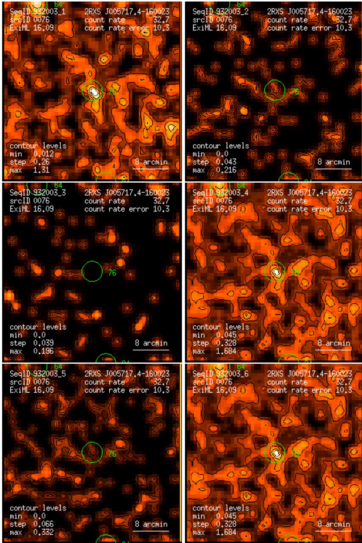
Figure 76: RASS 932003: detection 0076: band rate images, Gaussian filter: (1) PSPC channels 11 – 41, (2) 52 – 90, (3) 91 – 201, (4) 11 – 235, (5) 52 – 201, (6) 11 – 201. Broad band rates in counts/ks. Band rate contour levels in counts/ks/arcmin 2 .
