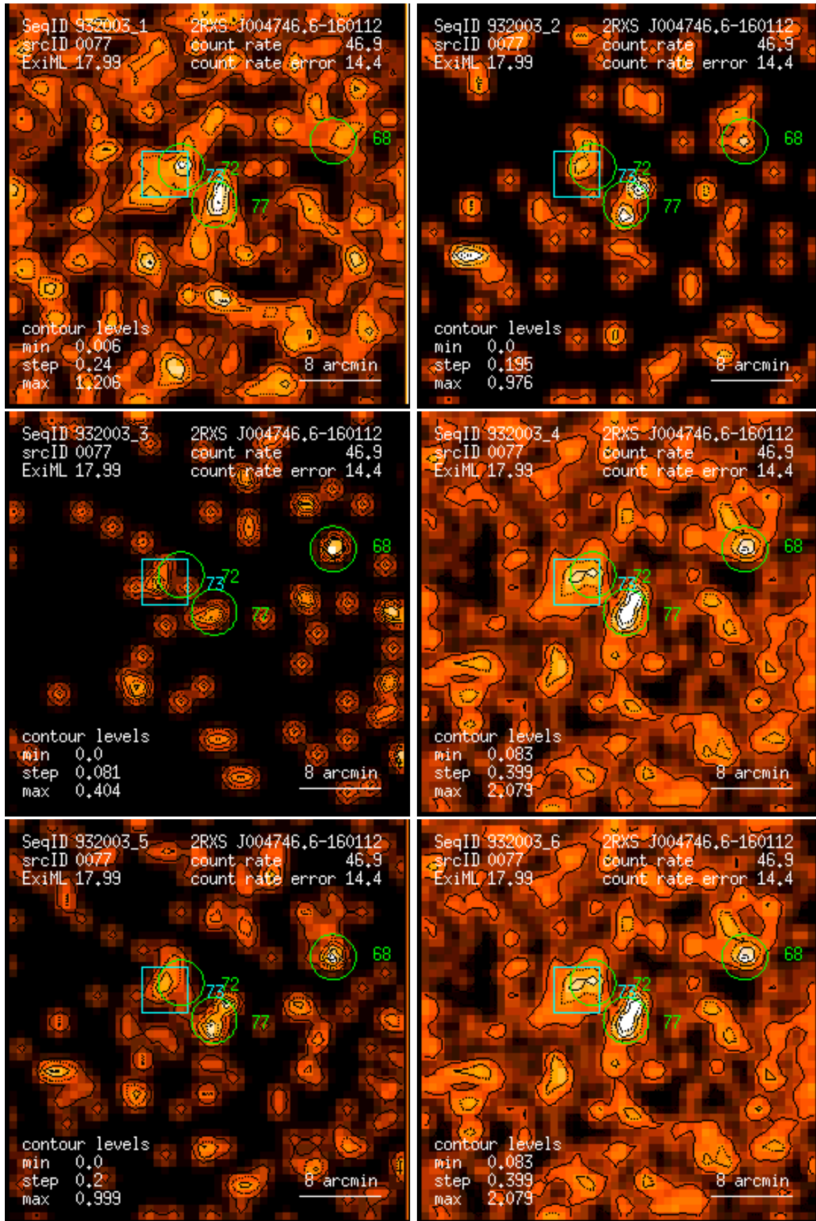
Figure 77: RASS 932003: detection 0077: band rate images, Gaussian filter: (1) PSPC channels 11 – 41, (2) 52 – 90, (3) 91 – 201, (4) 11 – 235, (5) 52 – 201, (6) 11 – 201. Broad band rates in counts/ks. Band rate contour levels in counts/ks/arcmin 2 .
