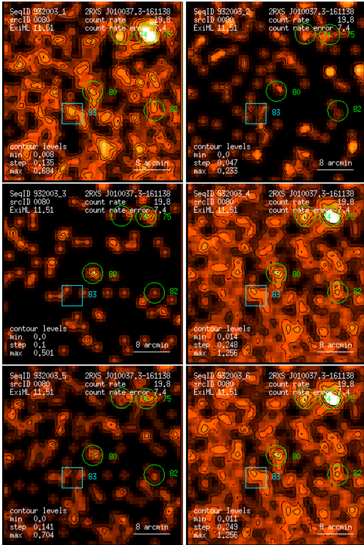
Figure 80: RASS 932003: detection 0080: band rate images, Gaussian filter: (1) PSPC channels 11 – 41, (2) 52 – 90, (3) 91 – 201, (4) 11 – 235, (5) 52 – 201, (6) 11 – 201. Broad band rates in counts/ks. Band rate contour levels in counts/ks/arcmin 2 .
