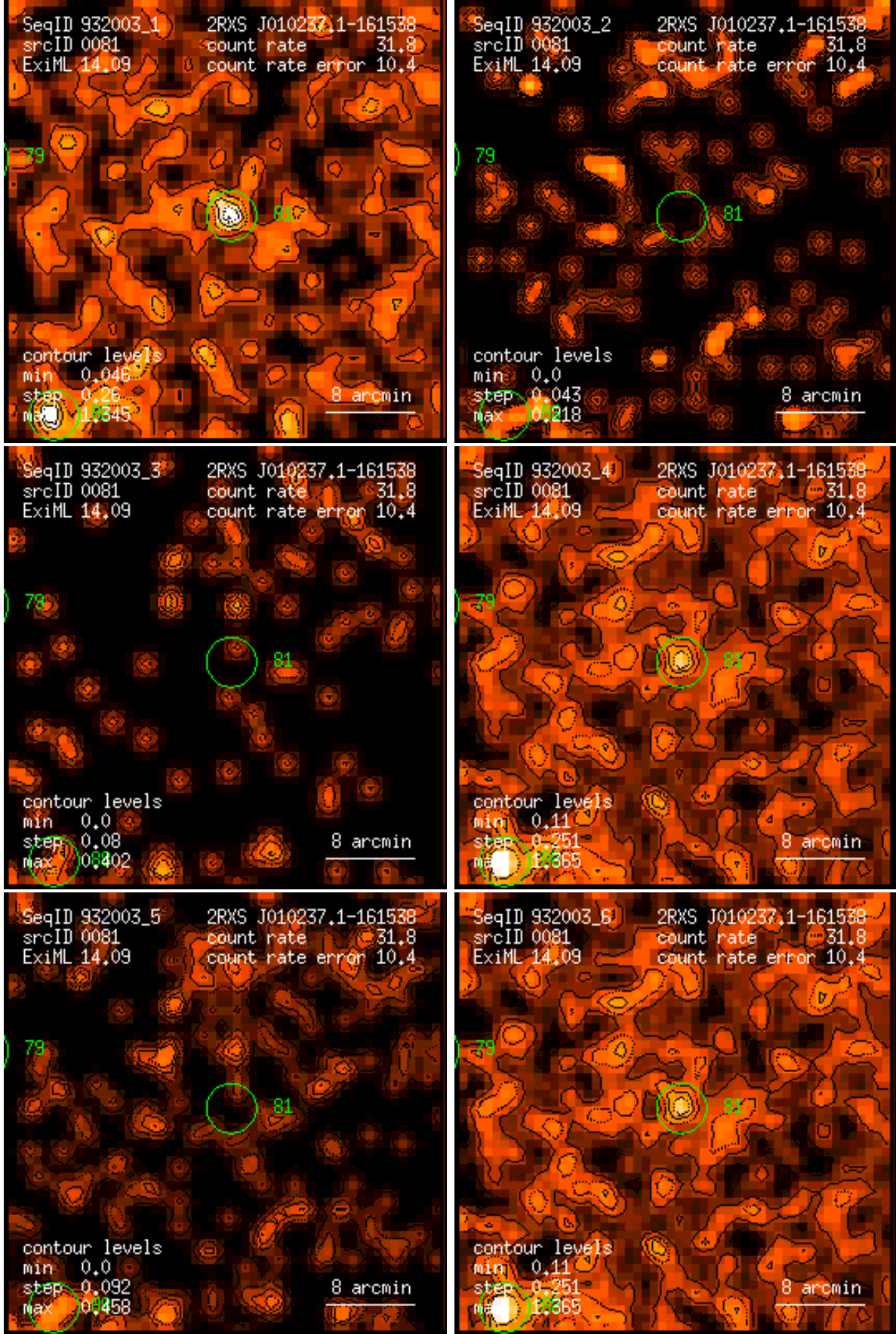
Figure 81: RASS 932003: detection 0081: band rate images, Gaussian filter: (1) PSPC channels 11 – 41, (2) 52 – 90, (3) 91 – 201, (4) 11 – 235, (5) 52 – 201, (6) 11 – 201. Broad band rates in counts/ks. Band rate contour levels in counts/ks/arcmin 2 .
