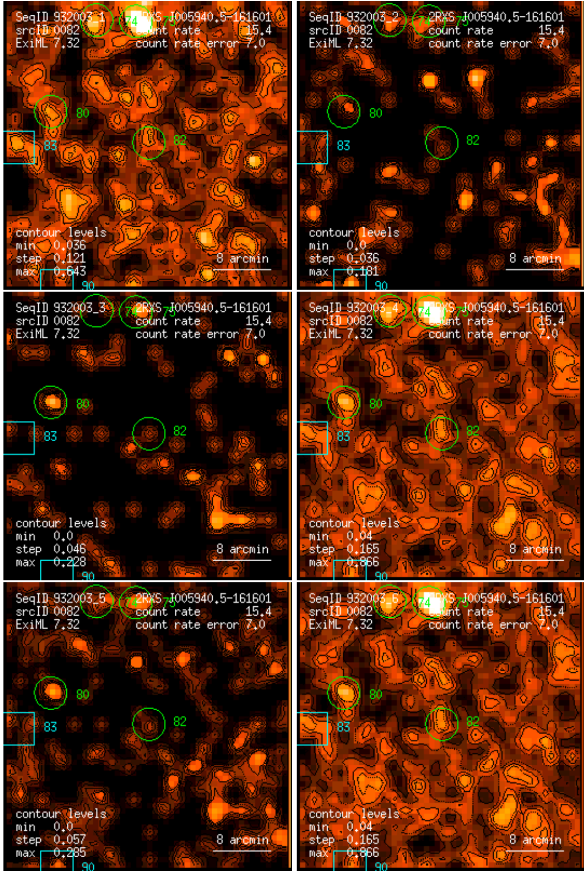
Figure 82: RASS 932003: detection 0082: band rate images, Gaussian filter: (1) PSPC channels 11 – 41, (2) 52 – 90, (3) 91 – 201, (4) 11 – 235, (5) 52 – 201, (6) 11 – 201. Broad band rates in counts/ks. Band rate contour levels in counts/ks/arcmin 2 .
