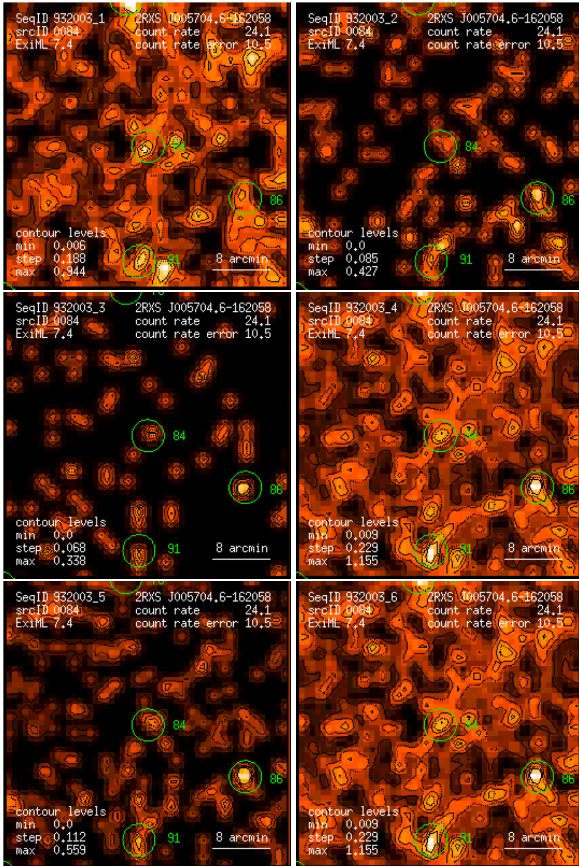
Figure 84: RASS 932003: detection 0084: band rate images, Gaussian filter: (1) PSPC channels 11 – 41, (2) 52 – 90, (3) 91 – 201, (4) 11 – 235, (5) 52 – 201, (6) 11 – 201. Broad band rates in counts/ks. Band rate contour levels in counts/ks/arcmin 2 .
