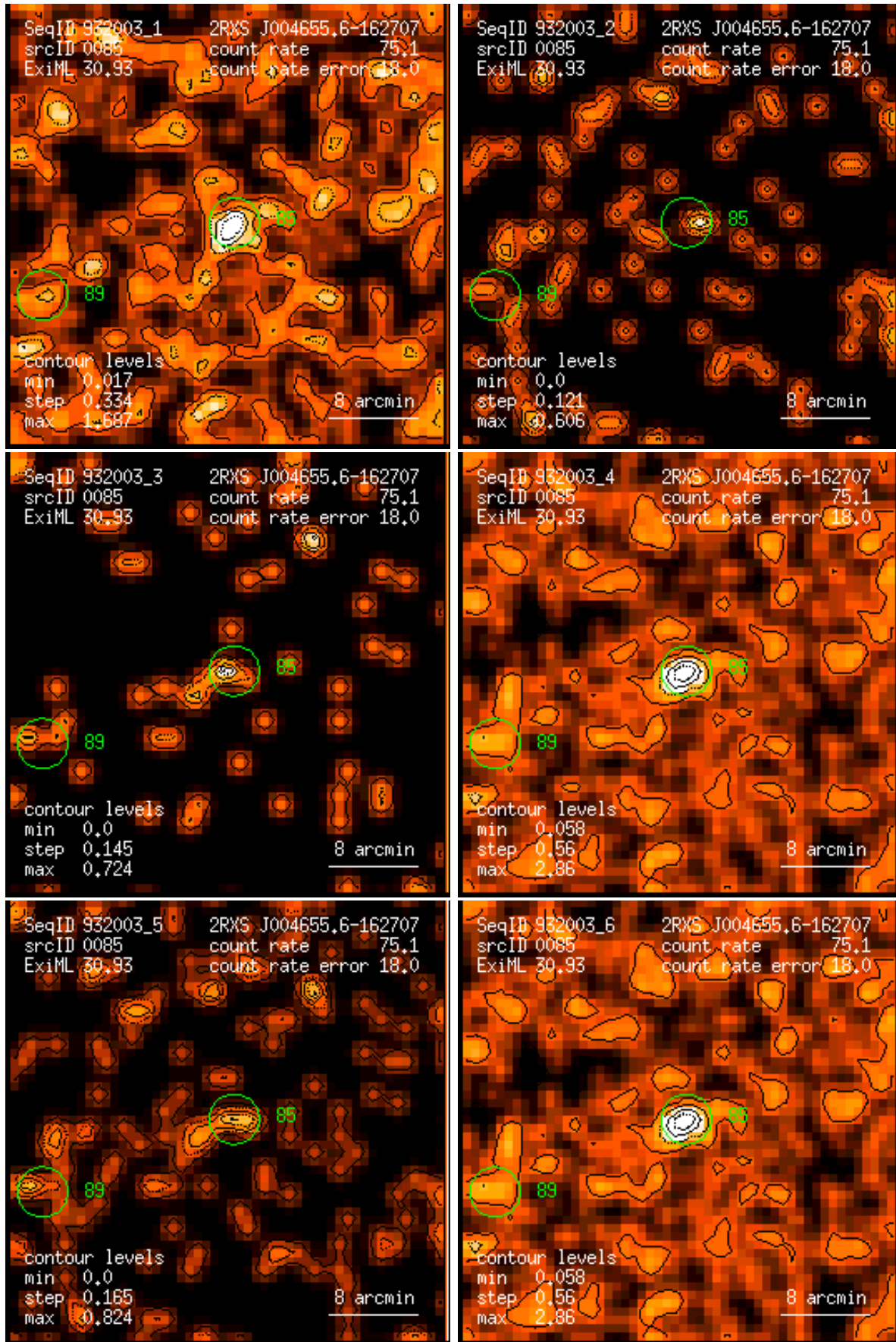
Figure 85: RASS 932003: detection 0085: band rate images, Gaussian filter: (1) PSPC channels 11 – 41, (2) 52 – 90, (3) 91 – 201, (4) 11 – 235, (5) 52 – 201, (6) 11 – 201. Broad band rates in counts/ks. Band rate contour levels in counts/ks/arcmin 2 .
