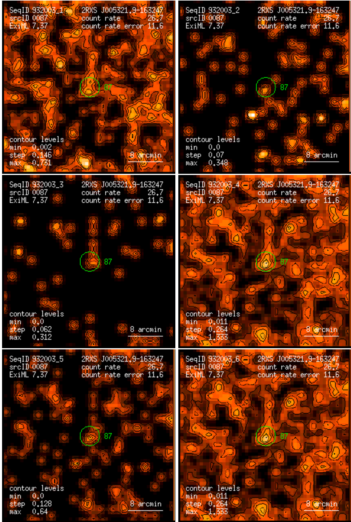
Figure 87: RASS 932003: detection 0087: band rate images, Gaussian filter: (1) PSPC channels 11 – 41, (2) 52 – 90, (3) 91 – 201, (4) 11 – 235, (5) 52 – 201, (6) 11 – 201. Broad band rates in counts/ks. Band rate contour levels in counts/ks/arcmin 2 .
