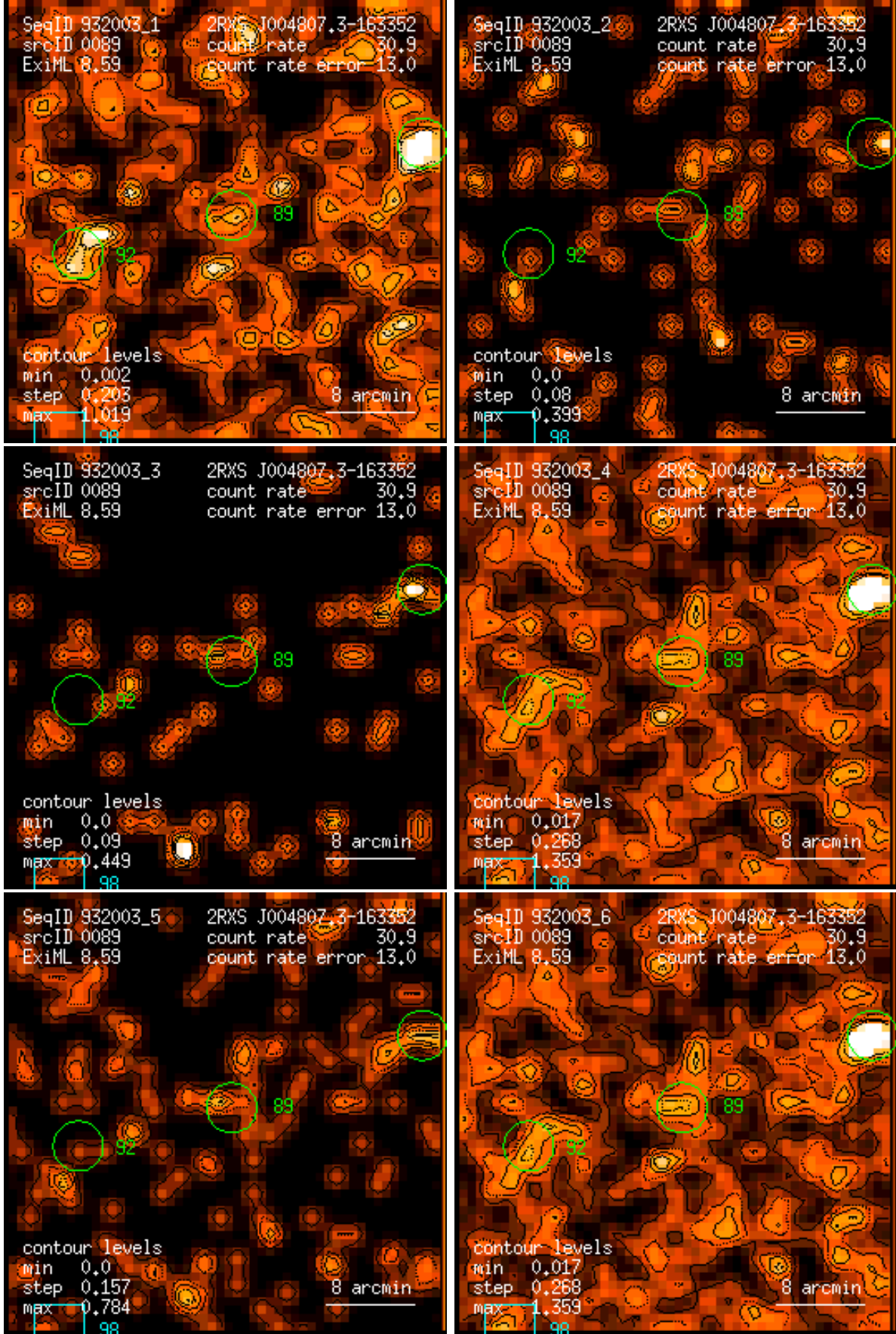
Figure 89: RASS 932003: detection 0089: band rate images, Gaussian filter: (1) PSPC channels 11 – 41, (2) 52 – 90, (3) 91 – 201, (4) 11 – 235, (5) 52 – 201, (6) 11 – 201. Broad band rates in counts/ks. Band rate contour levels in counts/ks/arcmin 2 .
