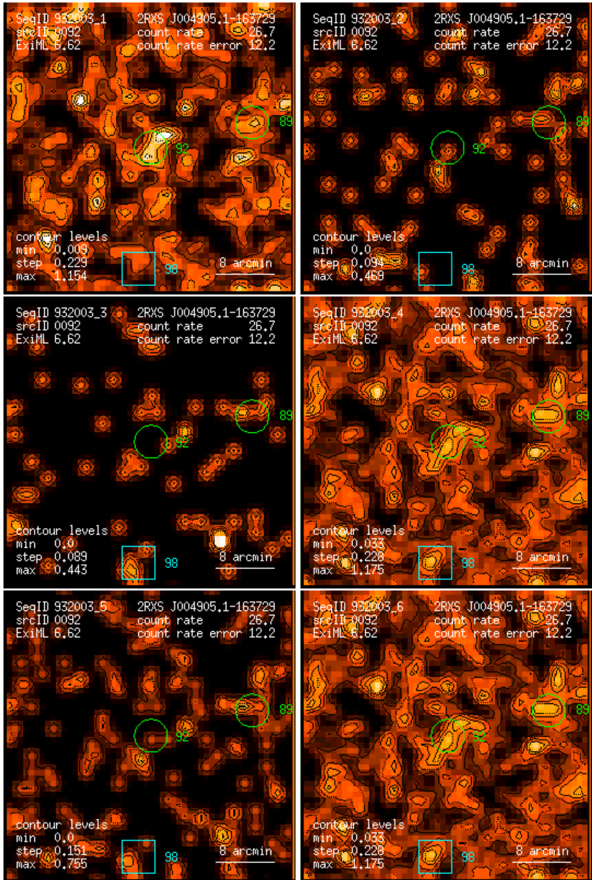
Figure 92: RASS 932003: detection 0092: band rate images, Gaussian filter: (1) PSPC channels 11 – 41, (2) 52 – 90, (3) 91 – 201, (4) 11 – 235, (5) 52 – 201, (6) 11 – 201. Broad band rates in counts/ks. Band rate contour levels in counts/ks/arcmin 2 .
