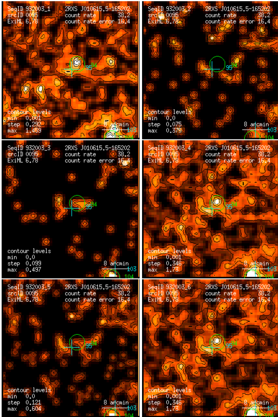
Figure 95: RASS 932003: detection 0095: band rate images, Gaussian filter: (1) PSPC channels 11 – 41, (2) 52 – 90, (3) 91 – 201, (4) 11 – 235, (5) 52 – 201, (6) 11 – 201. Broad band rates in counts/ks. Band rate contour levels in counts/ks/arcmin 2 .
