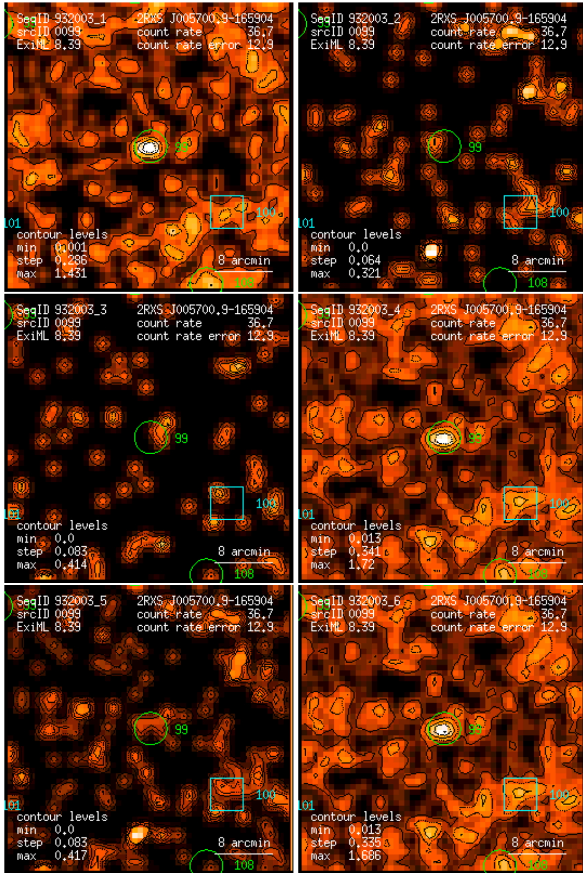
Figure 99: RASS 932003: detection 0099: band rate images, Gaussian filter: (1) PSPC channels 11 – 41, (2) 52 – 90, (3) 91 – 201, (4) 11 – 235, (5) 52 – 201, (6) 11 – 201. Broad band rates in counts/ks. Band rate contour levels in counts/ks/arcmin 2 .
