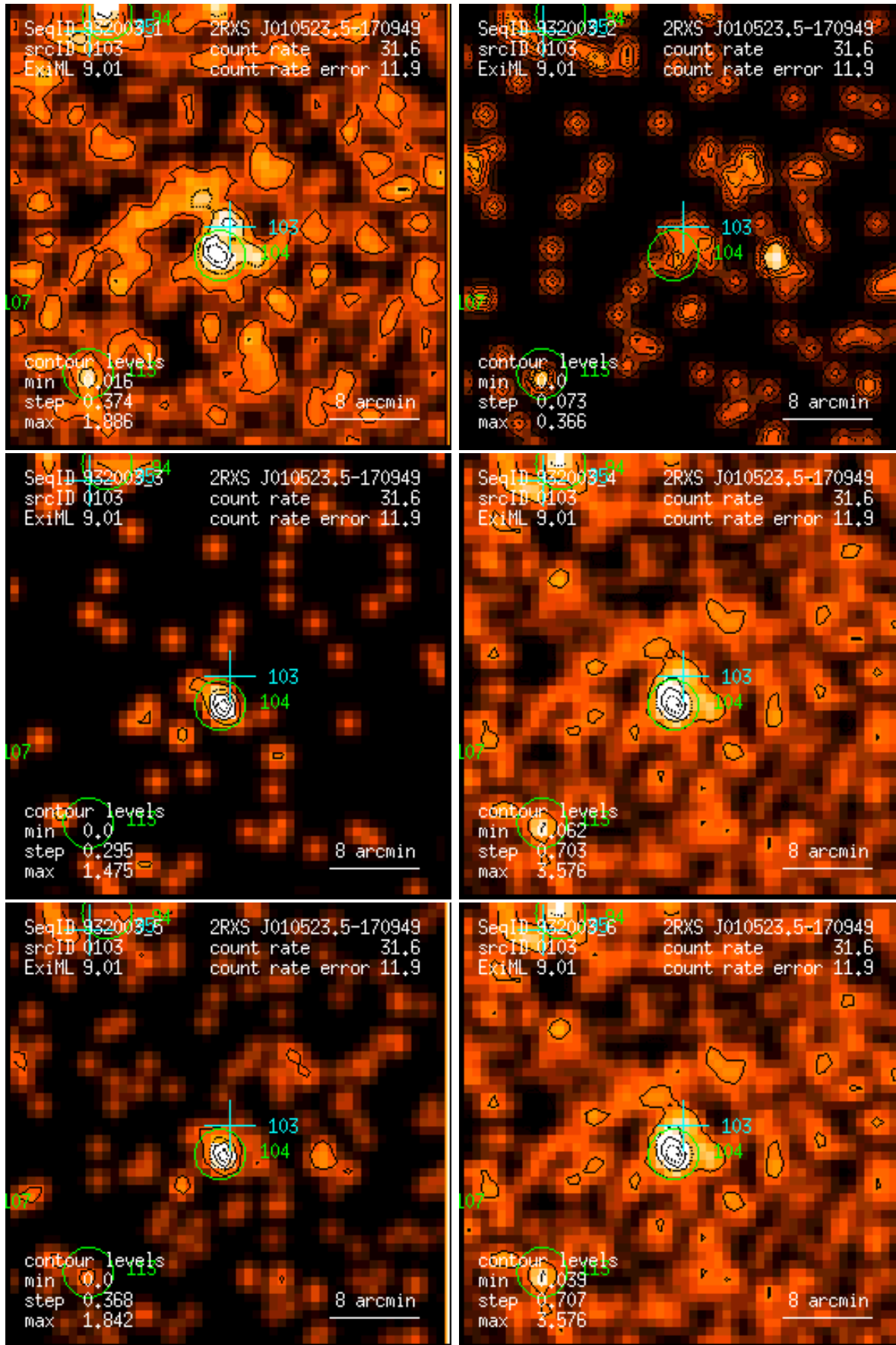
Figure 103: RASS 932003: detection 0103: band rate images, Gaussian filter: (1) PSPC channels 11 – 41, (2) 52 – 90, (3) 91 – 201, (4) 11 – 235, (5) 52 – 201, (6) 11 – 201. Broad band rates in counts/ks. Band rate contour levels in counts/ks/arcmin 2 .
