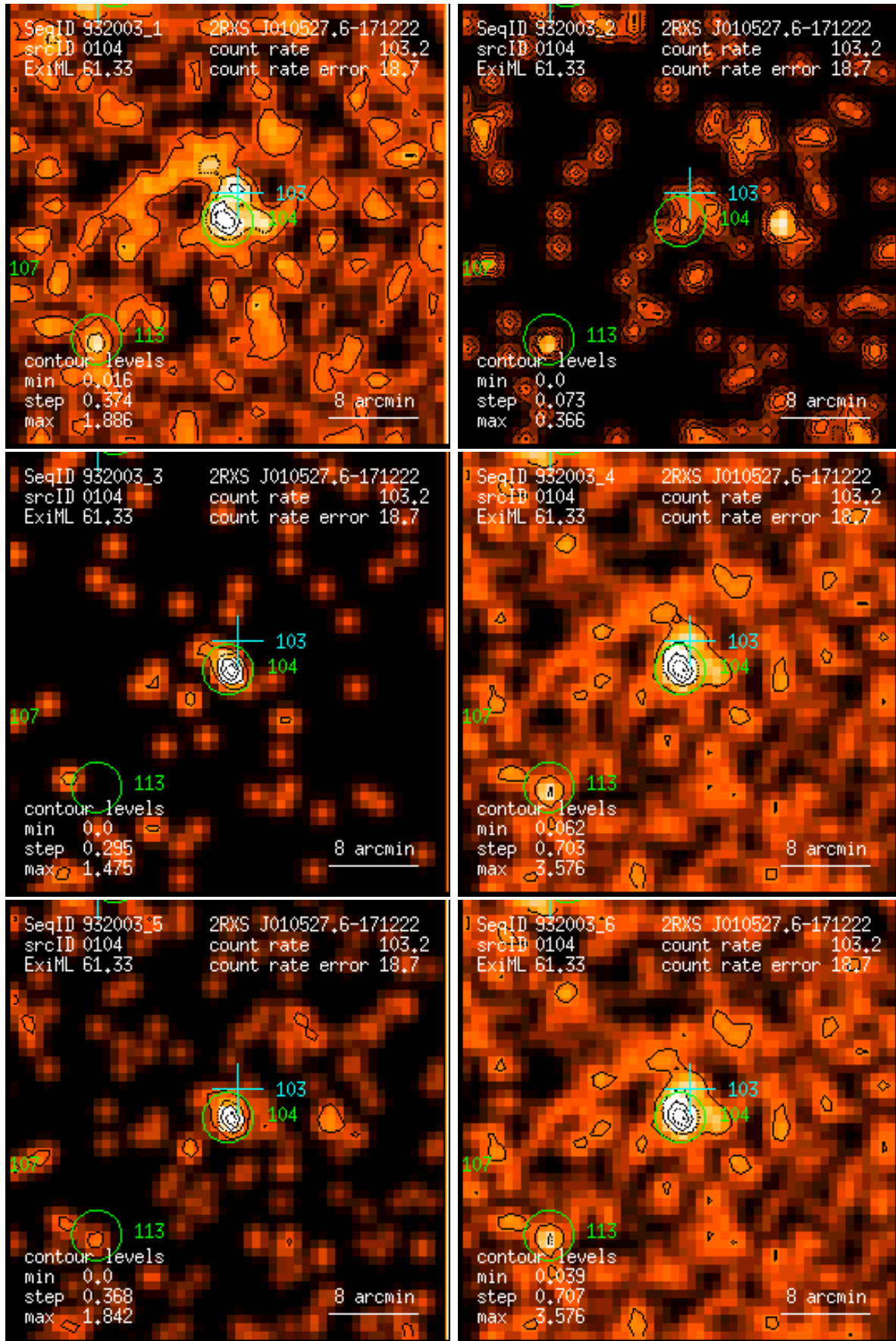
Figure 104: RASS 932003: detection 0104: band rate images, Gaussian filter: (1) PSPC channels 11 – 41, (2) 52 – 90, (3) 91 – 201, (4) 11 – 235, (5) 52 – 201, (6) 11 – 201. Broad band rates in counts/ks. Band rate contour levels in counts/ks/arcmin 2 .
