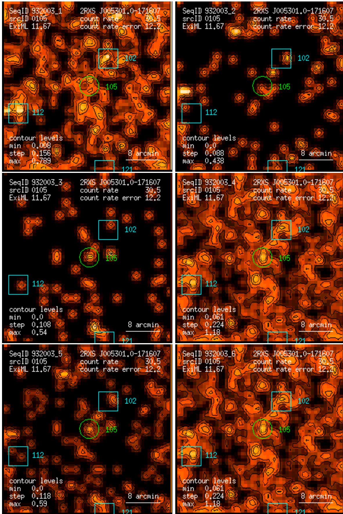
Figure 105: RASS 932003: detection 0105: band rate images, Gaussian filter: (1) PSPC channels 11 – 41, (2) 52 – 90, (3) 91 – 201, (4) 11 – 235, (5) 52 – 201, (6) 11 – 201. Broad band rates in counts/ks. Band rate contour levels in counts/ks/arcmin 2 .
