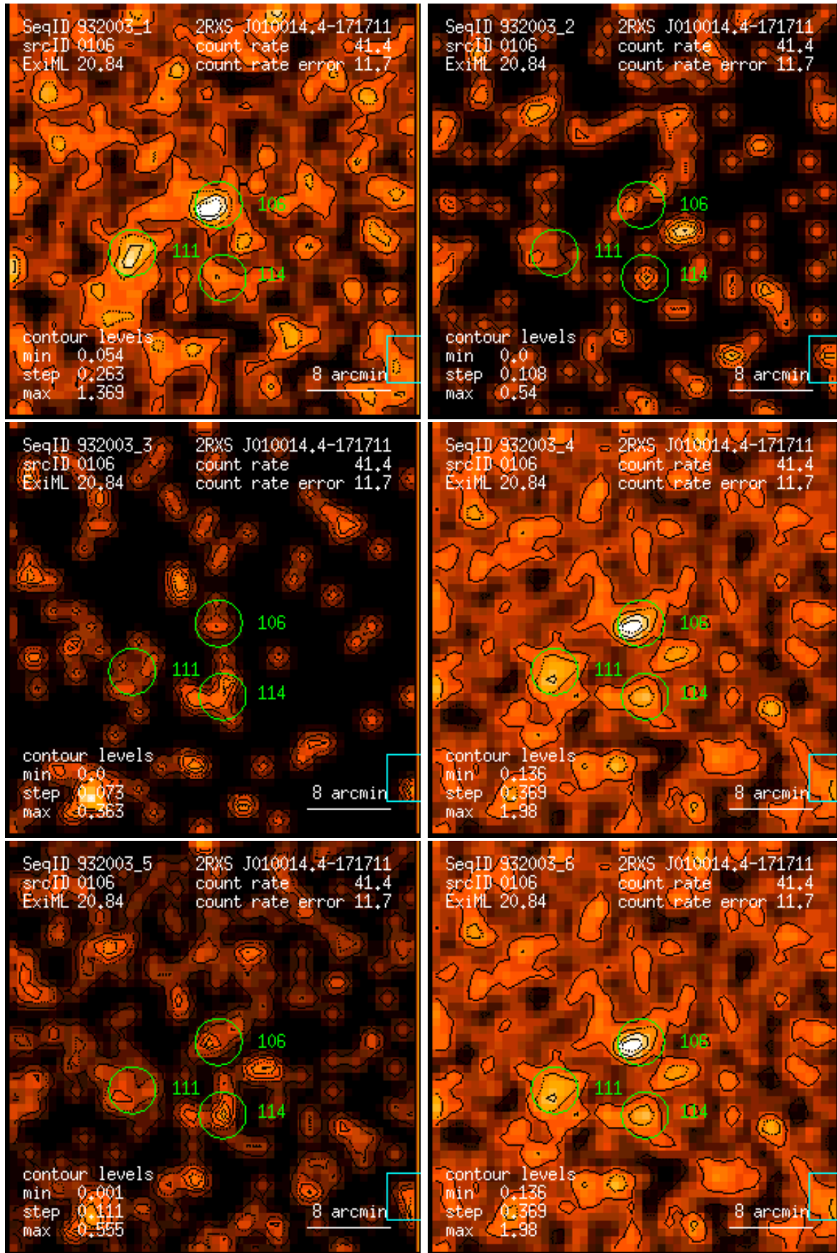
Figure 106: RASS 932003: detection 0106: band rate images, Gaussian filter: (1) PSPC channels 11 – 41, (2) 52 – 90, (3) 91 – 201, (4) 11 – 235, (5) 52 – 201, (6) 11 – 201. Broad band rates in counts/ks. Band rate contour levels in counts/ks/arcmin 2 .
