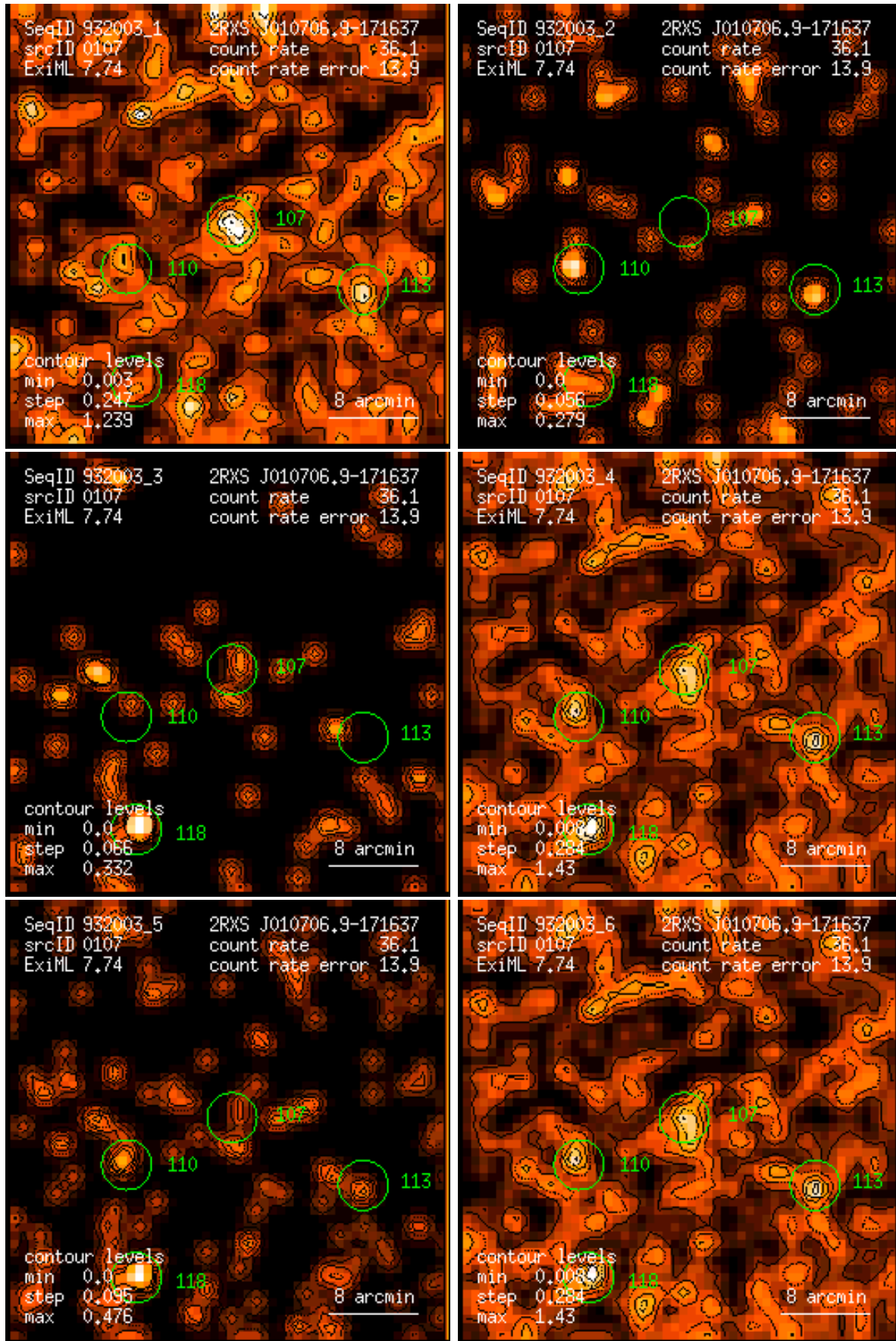
Figure 107: RASS 932003: detection 0107: band rate images, Gaussian filter: (1) PSPC channels 11 – 41, (2) 52 – 90, (3) 91 – 201, (4) 11 – 235, (5) 52 – 201, (6) 11 – 201. Broad band rates in counts/ks. Band rate contour levels in counts/ks/arcmin 2 .
