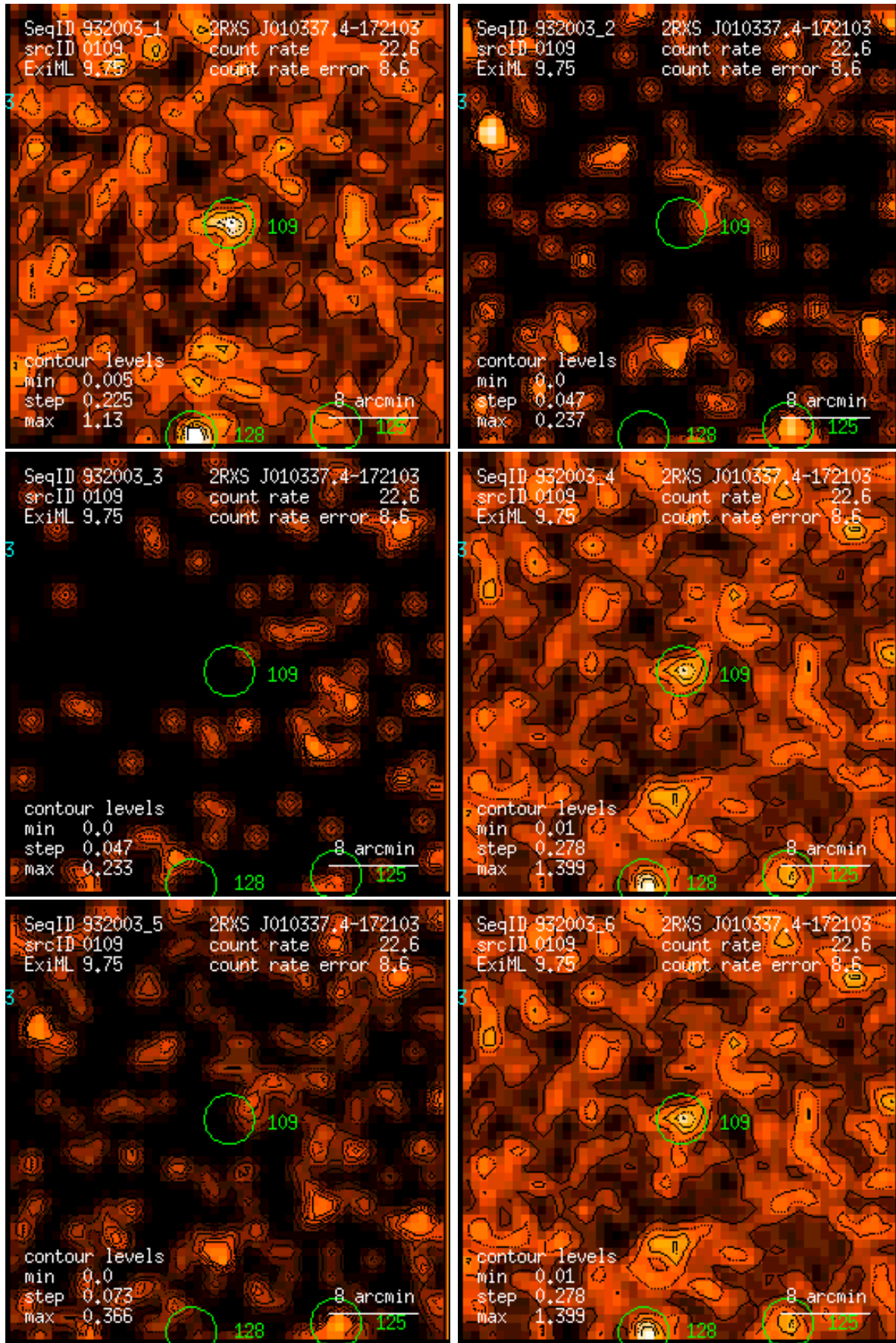
Figure 109: RASS 932003: detection 0109: band rate images, Gaussian filter: (1) PSPC channels 11 – 41, (2) 52 – 90, (3) 91 – 201, (4) 11 – 235, (5) 52 – 201, (6) 11 – 201. Broad band rates in counts/ks. Band rate contour levels in counts/ks/arcmin 2 .
