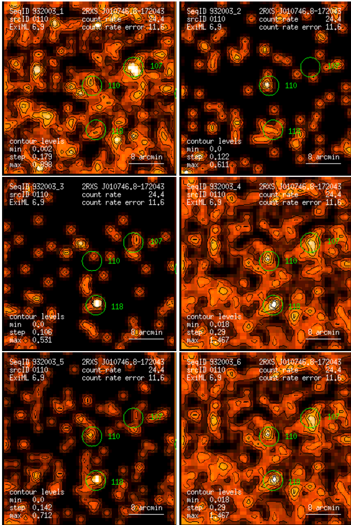
Figure 110: RASS 932003: detection 0110: band rate images, Gaussian filter: (1) PSPC channels 11 – 41, (2) 52 – 90, (3) 91 – 201, (4) 11 – 235, (5) 52 – 201, (6) 11 – 201. Broad band rates in counts/ks. Band rate contour levels in counts/ks/arcmin 2 .
