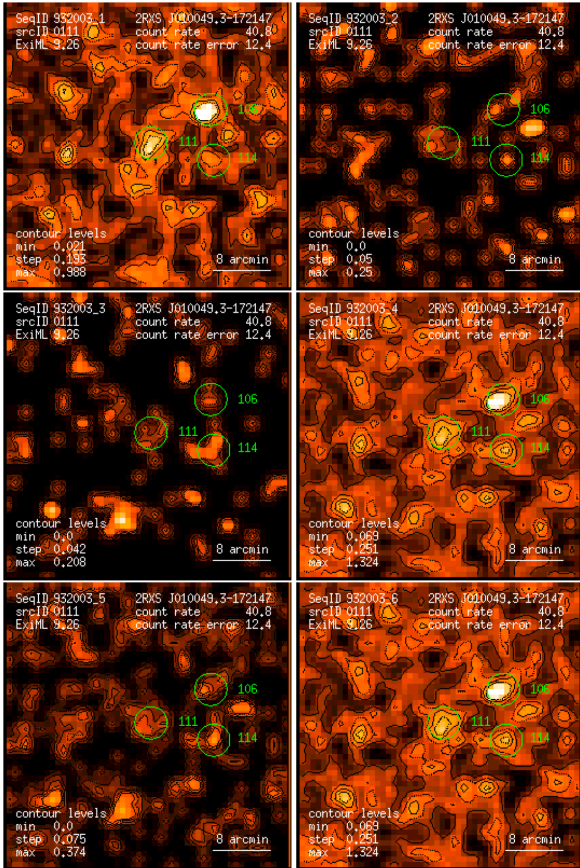
Figure 111: RASS 932003: detection 0111: band rate images, Gaussian filter: (1) PSPC channels 11 – 41, (2) 52 – 90, (3) 91 – 201, (4) 11 – 235, (5) 52 – 201, (6) 11 – 201. Broad band rates in counts/ks. Band rate contour levels in counts/ks/arcmin 2 .
