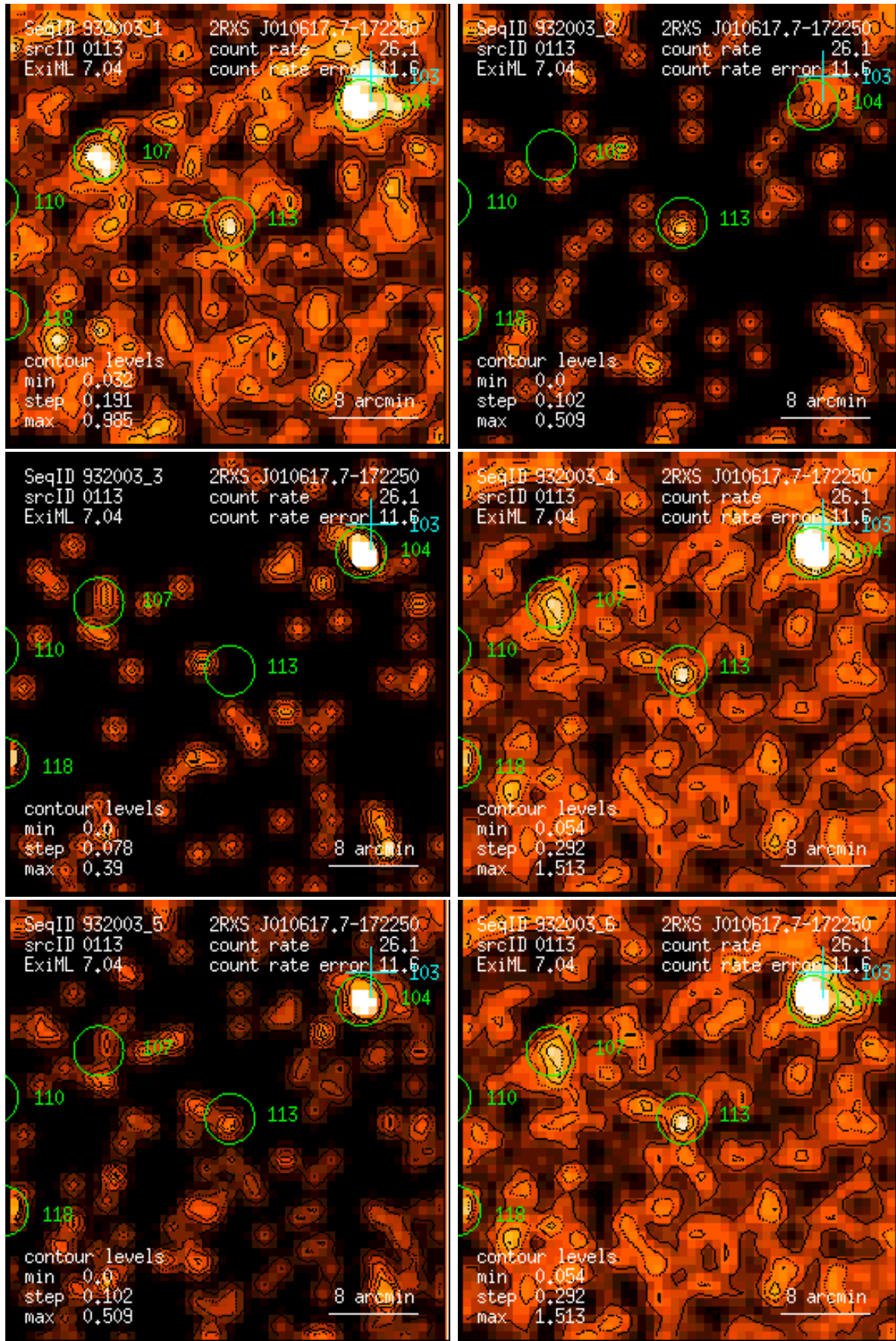
Figure 113: RASS 932003: detection 0113: band rate images, Gaussian filter: (1) PSPC channels 11 – 41, (2) 52 – 90, (3) 91 – 201, (4) 11 – 235, (5) 52 – 201, (6) 11 – 201. Broad band rates in counts/ks. Band rate contour levels in counts/ks/arcmin 2 .
