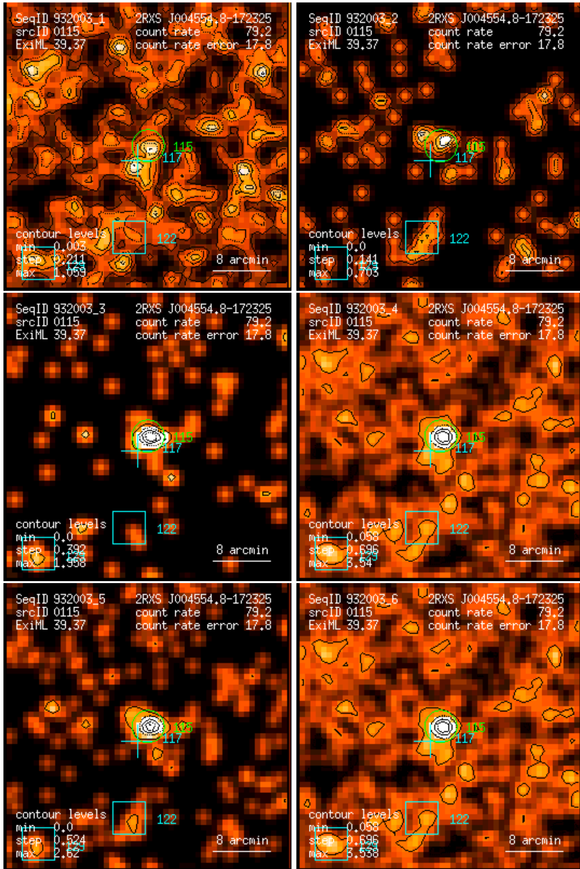
Figure 115: RASS 932003: detection 0115: band rate images, Gaussian filter: (1) PSPC channels 11 – 41, (2) 52 – 90, (3) 91 – 201, (4) 11 – 235, (5) 52 – 201, (6) 11 – 201. Broad band rates in counts/ks. Band rate contour levels in counts/ks/arcmin 2 .
