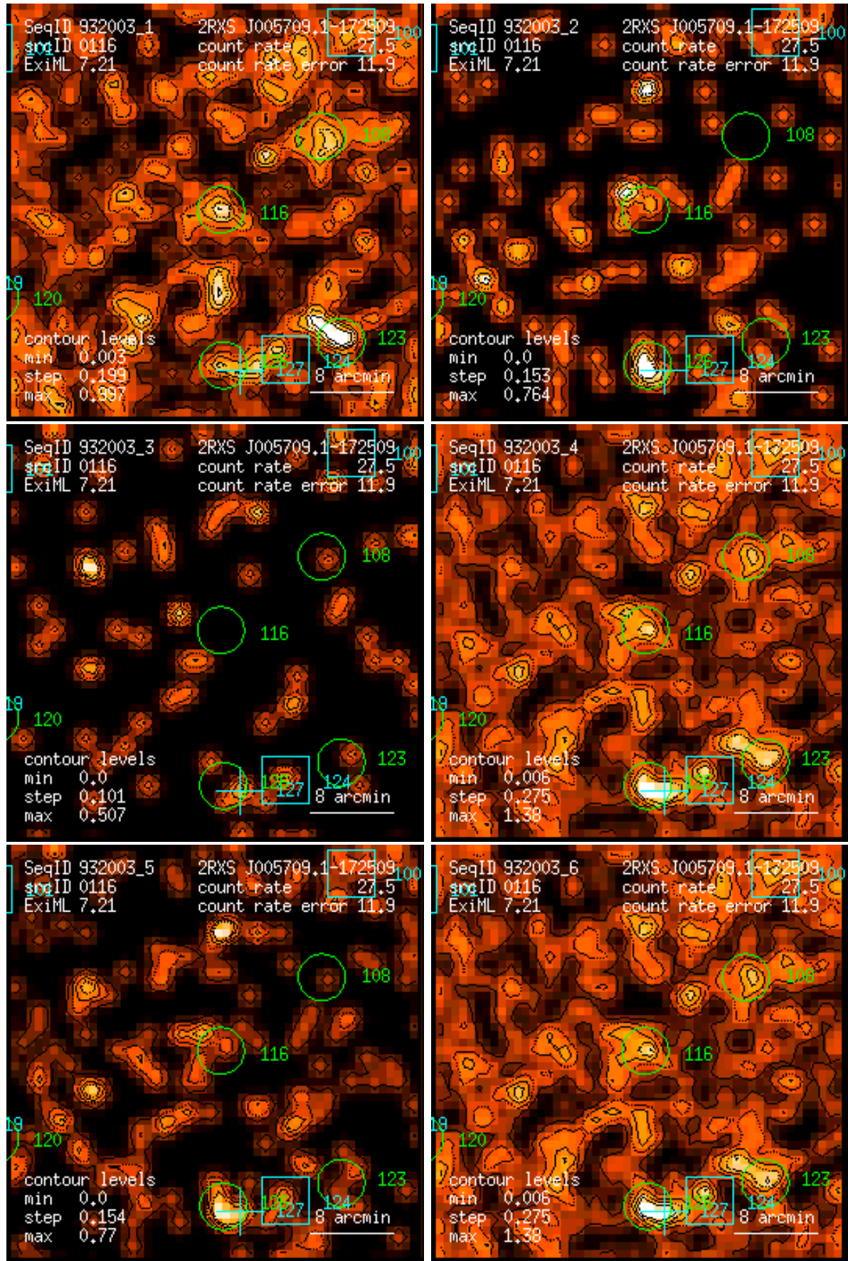
Figure 116: RASS 932003: detection 0116: band rate images, Gaussian filter: (1) PSPC channels 11 – 41, (2) 52 – 90, (3) 91 – 201, (4) 11 – 235, (5) 52 – 201, (6) 11 – 201. Broad band rates in counts/ks. Band rate contour levels in counts/ks/arcmin 2 .
