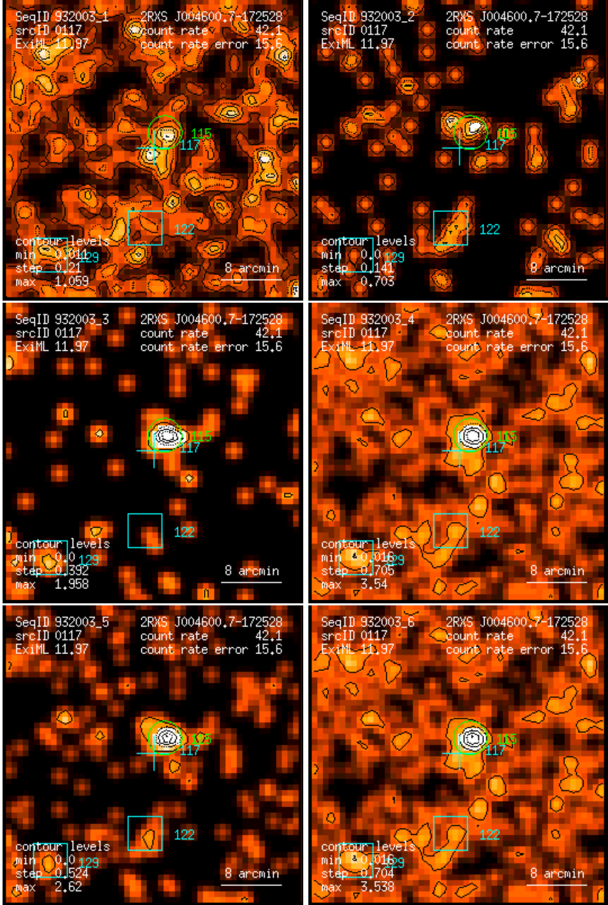
Figure 117: RASS 932003: detection 0117: band rate images, Gaussian filter: (1) PSPC channels 11 – 41, (2) 52 – 90, (3) 91 – 201, (4) 11 – 235, (5) 52 – 201, (6) 11 – 201. Broad band rates in counts/ks. Band rate contour levels in counts/ks/arcmin 2 .
