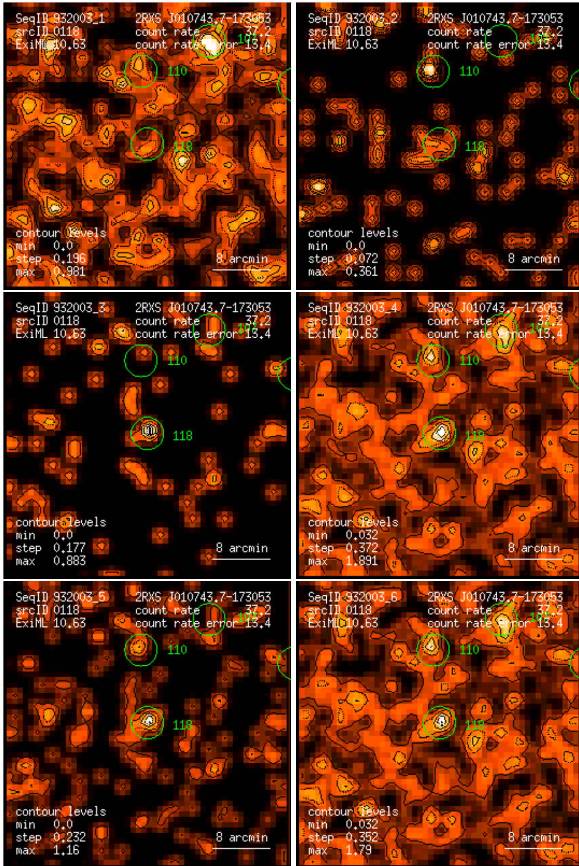
Figure 118: RASS 932003: detection 0118: band rate images, Gaussian filter: (1) PSPC channels 11 – 41, (2) 52 – 90, (3) 91 – 201, (4) 11 – 235, (5) 52 – 201, (6) 11 – 201. Broad band rates in counts/ks. Band rate contour levels in counts/ks/arcmin 2 .
