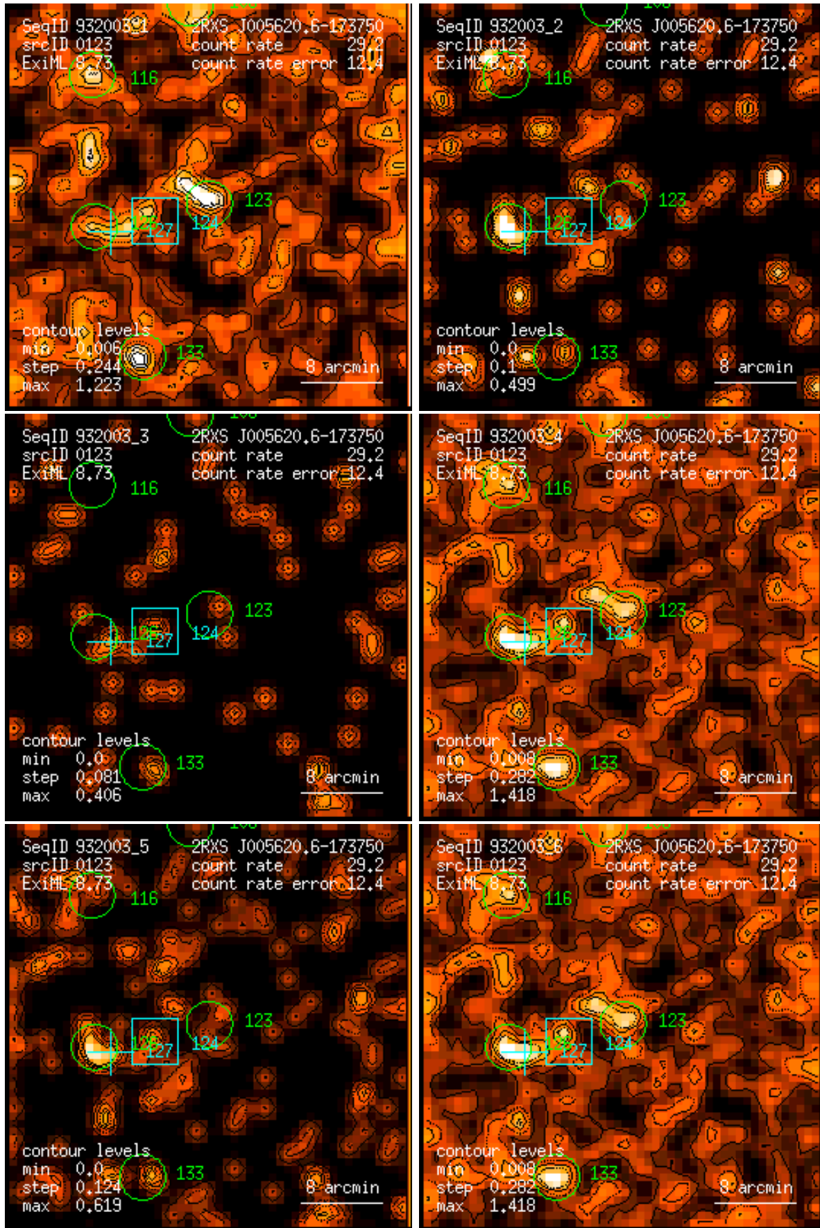
Figure 123: RASS 932003: detection 0123: band rate images, Gaussian filter: (1) PSPC channels 11 – 41, (2) 52 – 90, (3) 91 – 201, (4) 11 – 235, (5) 52 – 201, (6) 11 – 201. Broad band rates in counts/ks. Band rate contour levels in counts/ks/arcmin 2 .
