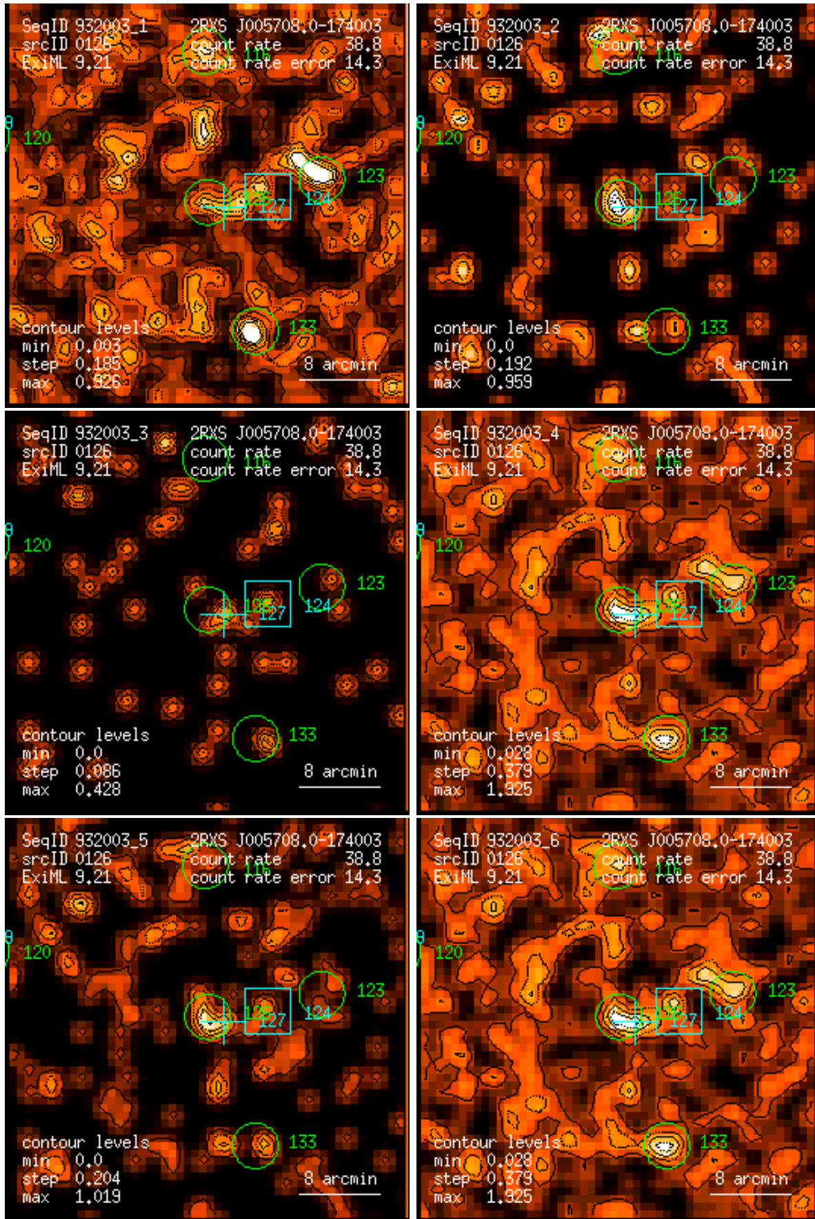
Figure 126: RASS 932003: detection 0126: band rate images, Gaussian filter: (1) PSPC channels 11 – 41, (2) 52 – 90, (3) 91 – 201, (4) 11 – 235, (5) 52 – 201, (6) 11 – 201. Broad band rates in counts/ks. Band rate contour levels in counts/ks/arcmin 2 .
