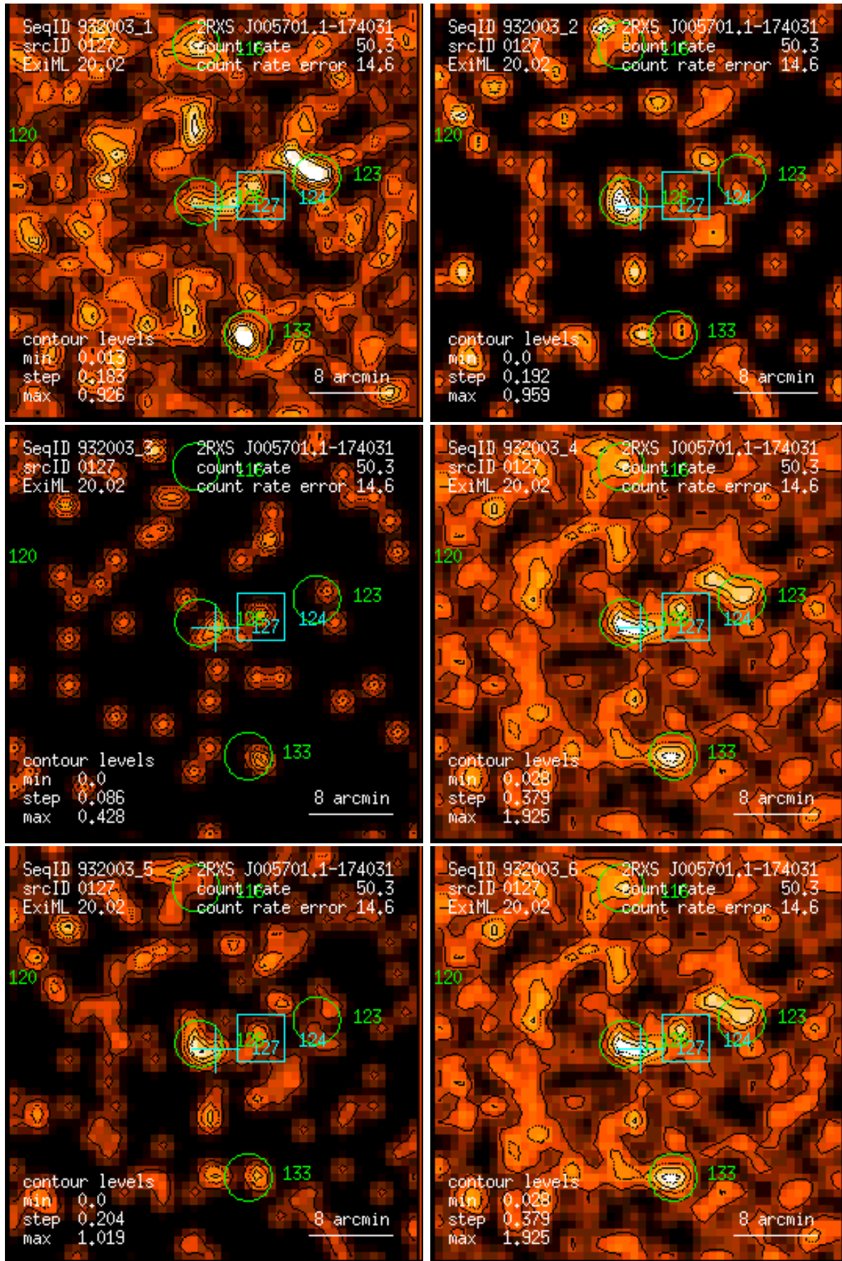
Figure 127: RASS 932003: detection 0127: band rate images, Gaussian filter: (1) PSPC channels 11 – 41, (2) 52 – 90, (3) 91 – 201, (4) 11 – 235, (5) 52 – 201, (6) 11 – 201. Broad band rates in counts/ks. Band rate contour levels in counts/ks/arcmin 2 .
