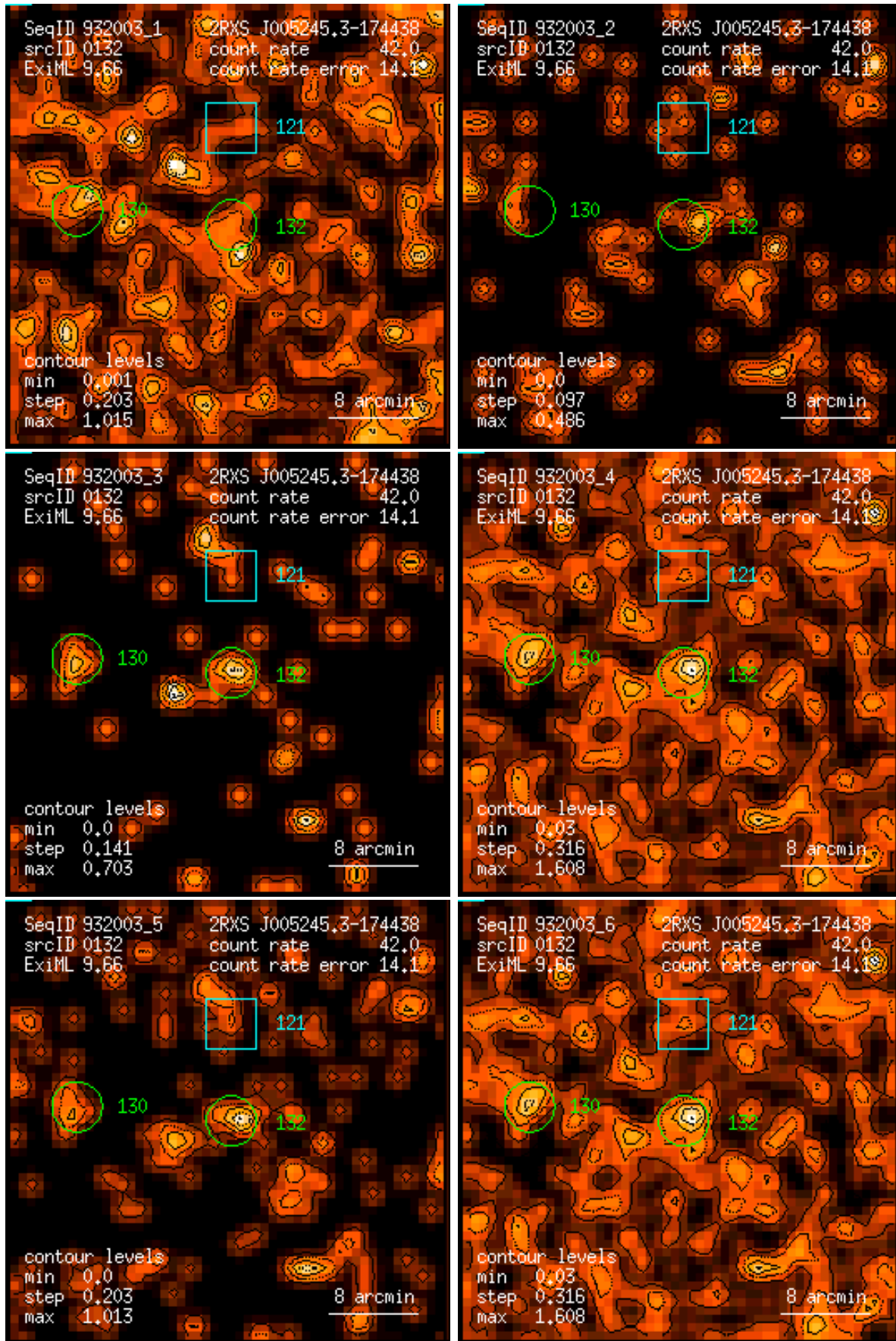
Figure 132: RASS 932003: detection 0132: band rate images, Gaussian filter: (1) PSPC channels 11 – 41, (2) 52 – 90, (3) 91 – 201, (4) 11 – 235, (5) 52 – 201, (6) 11 – 201. Broad band rates in counts/ks. Band rate contour levels in counts/ks/arcmin 2 .
