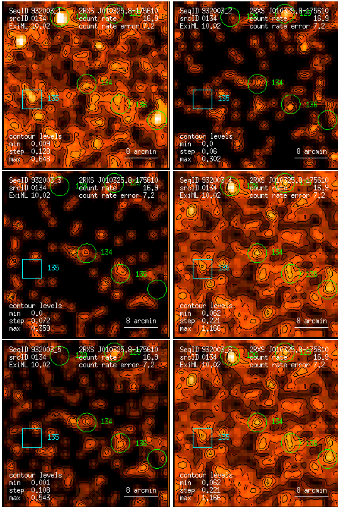
Figure 134: RASS 932003: detection 0134: band rate images, Gaussian filter: (1) PSPC channels 11 – 41, (2) 52 – 90, (3) 91 – 201, (4) 11 – 235, (5) 52 – 201, (6) 11 – 201. Broad band rates in counts/ks. Band rate contour levels in counts/ks/arcmin 2 .
