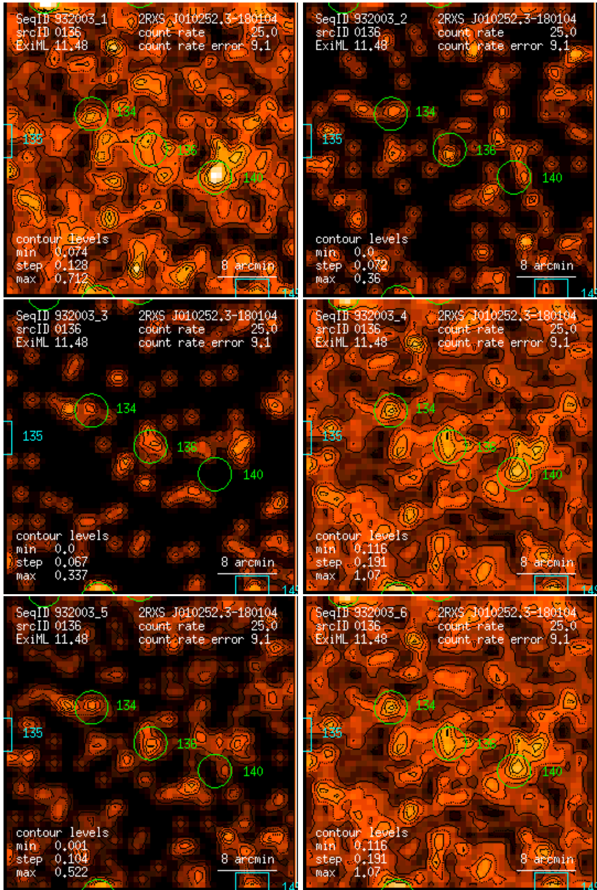
Figure 136: RASS 932003: detection 0136: band rate images, Gaussian filter: (1) PSPC channels 11 – 41, (2) 52 – 90, (3) 91 – 201, (4) 11 – 235, (5) 52 – 201, (6) 11 – 201. Broad band rates in counts/ks. Band rate contour levels in counts/ks/arcmin 2 .
