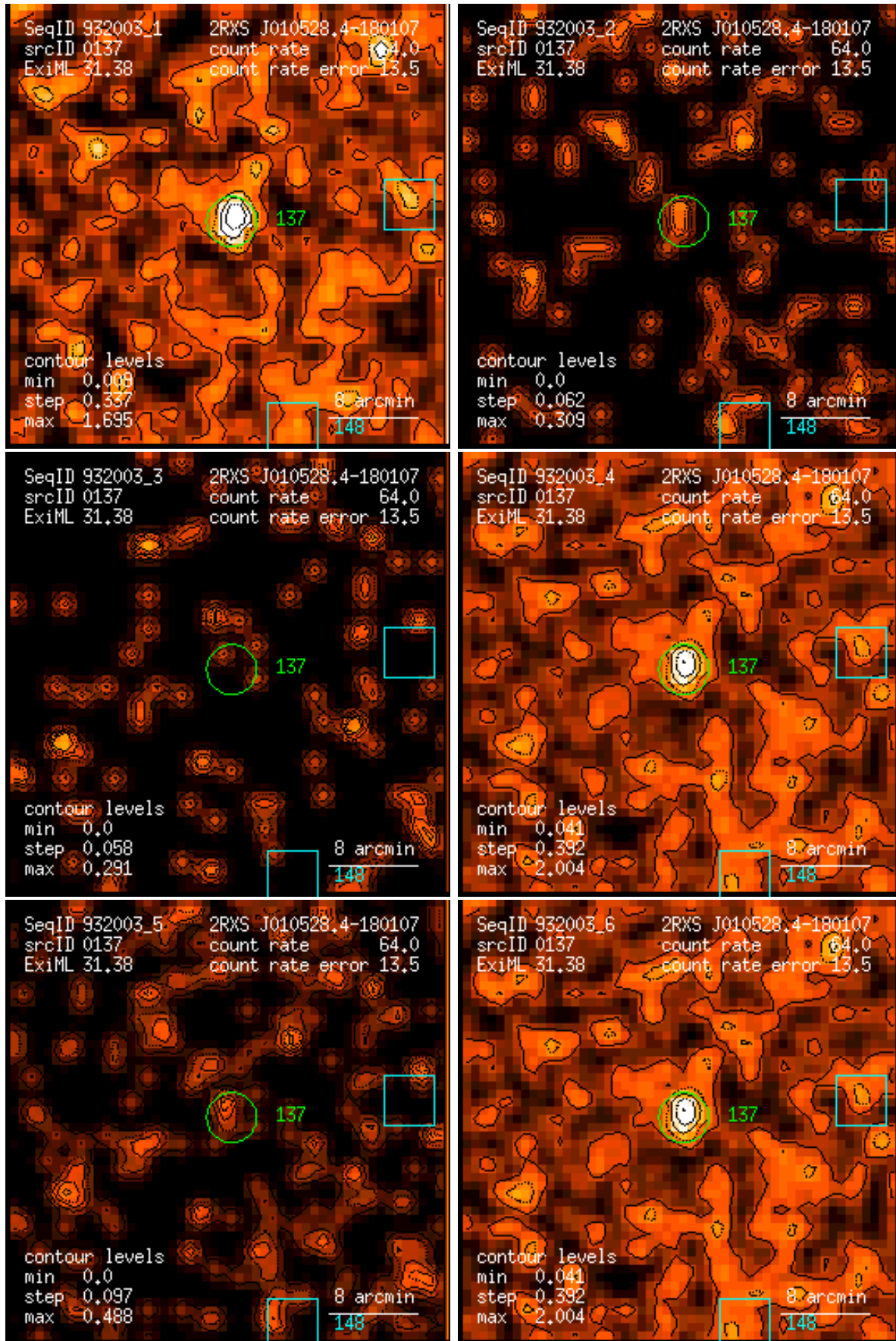
Figure 137: RASS 932003: detection 0137: band rate images, Gaussian filter: (1) PSPC channels 11 – 41, (2) 52 – 90, (3) 91 – 201, (4) 11 – 235, (5) 52 – 201, (6) 11 – 201. Broad band rates in counts/ks. Band rate contour levels in counts/ks/arcmin 2 .
