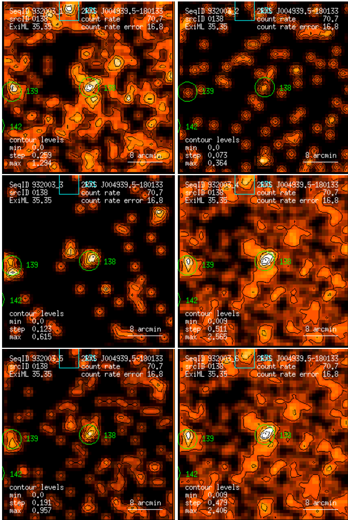
Figure 138: RASS 932003: detection 0138: band rate images, Gaussian filter: (1) PSPC channels 11 – 41, (2) 52 – 90, (3) 91 – 201, (4) 11 – 235, (5) 52 – 201, (6) 11 – 201. Broad band rates in counts/ks. Band rate contour levels in counts/ks/arcmin 2 .
