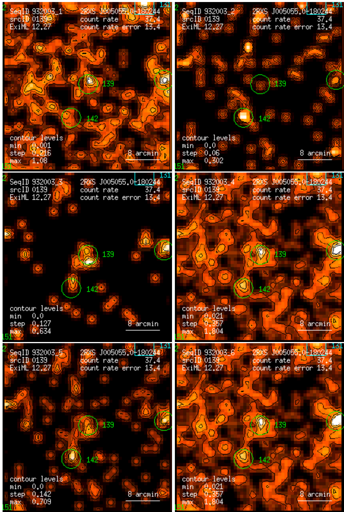
Figure 139: RASS 932003: detection 0139: band rate images, Gaussian filter: (1) PSPC channels 11 – 41, (2) 52 – 90, (3) 91 – 201, (4) 11 – 235, (5) 52 – 201, (6) 11 – 201. Broad band rates in counts/ks. Band rate contour levels in counts/ks/arcmin 2 .
