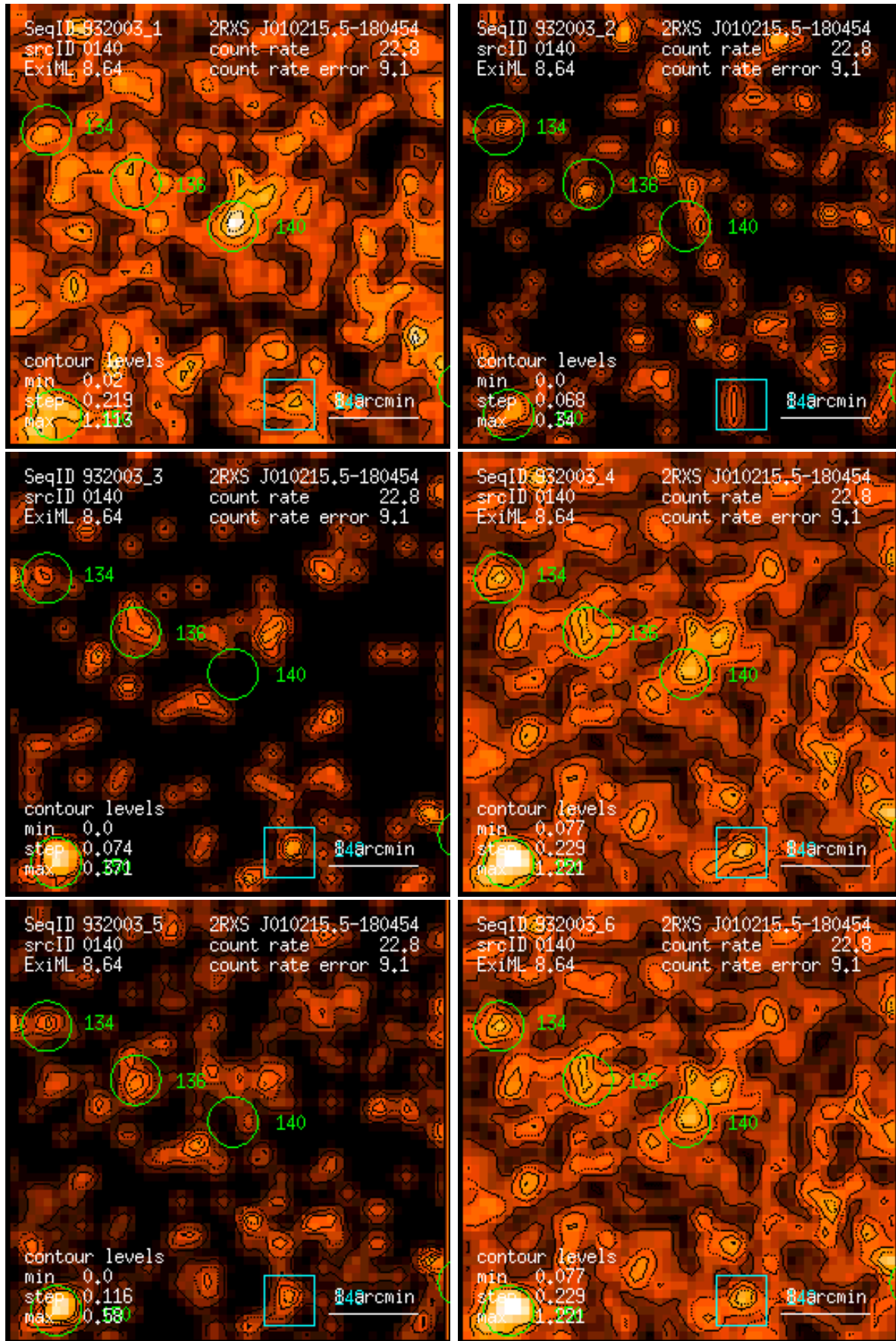
Figure 140: RASS 932003: detection 0140: band rate images, Gaussian filter: (1) PSPC channels 11 – 41, (2) 52 – 90, (3) 91 – 201, (4) 11 – 235, (5) 52 – 201, (6) 11 – 201. Broad band rates in counts/ks. Band rate contour levels in counts/ks/arcmin 2 .
