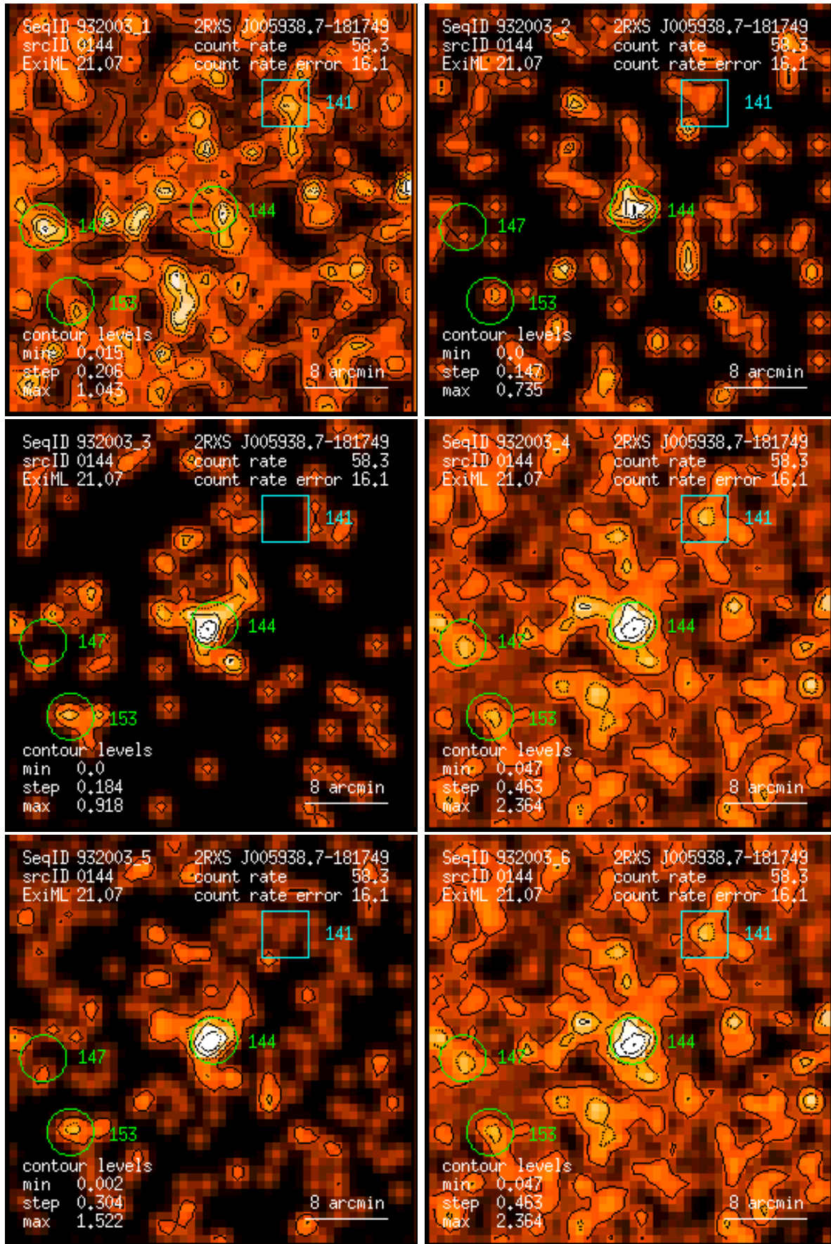
Figure 144: RASS 932003: detection 0144: band rate images, Gaussian filter: (1) PSPC channels 11 – 41, (2) 52 – 90, (3) 91 – 201, (4) 11 – 235, (5) 52 – 201, (6) 11 – 201. Broad band rates in counts/ks. Band rate contour levels in counts/ks/arcmin 2 .
