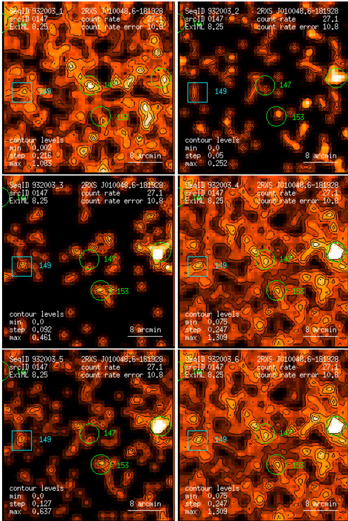
Figure 147: RASS 932003: detection 0147: band rate images, Gaussian filter: (1) PSPC channels 11 – 41, (2) 52 – 90, (3) 91 – 201, (4) 11 – 235, (5) 52 – 201, (6) 11 – 201. Broad band rates in counts/ks. Band rate contour levels in counts/ks/arcmin 2 .
