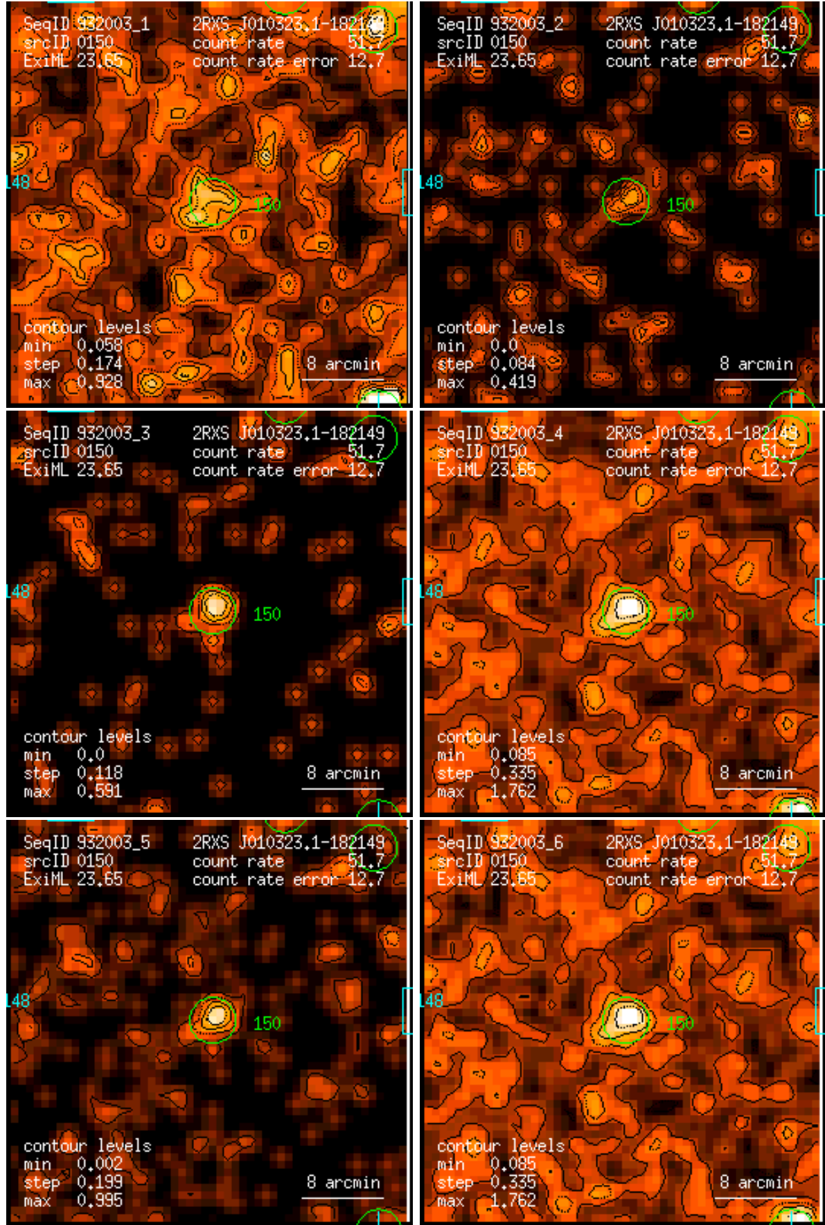
Figure 150: RASS 932003: detection 0150: band rate images, Gaussian filter: (1) PSPC channels 11 – 41, (2) 52 – 90, (3) 91 – 201, (4) 11 – 235, (5) 52 – 201, (6) 11 – 201. Broad band rates in counts/ks. Band rate contour levels in counts/ks/arcmin 2 .
