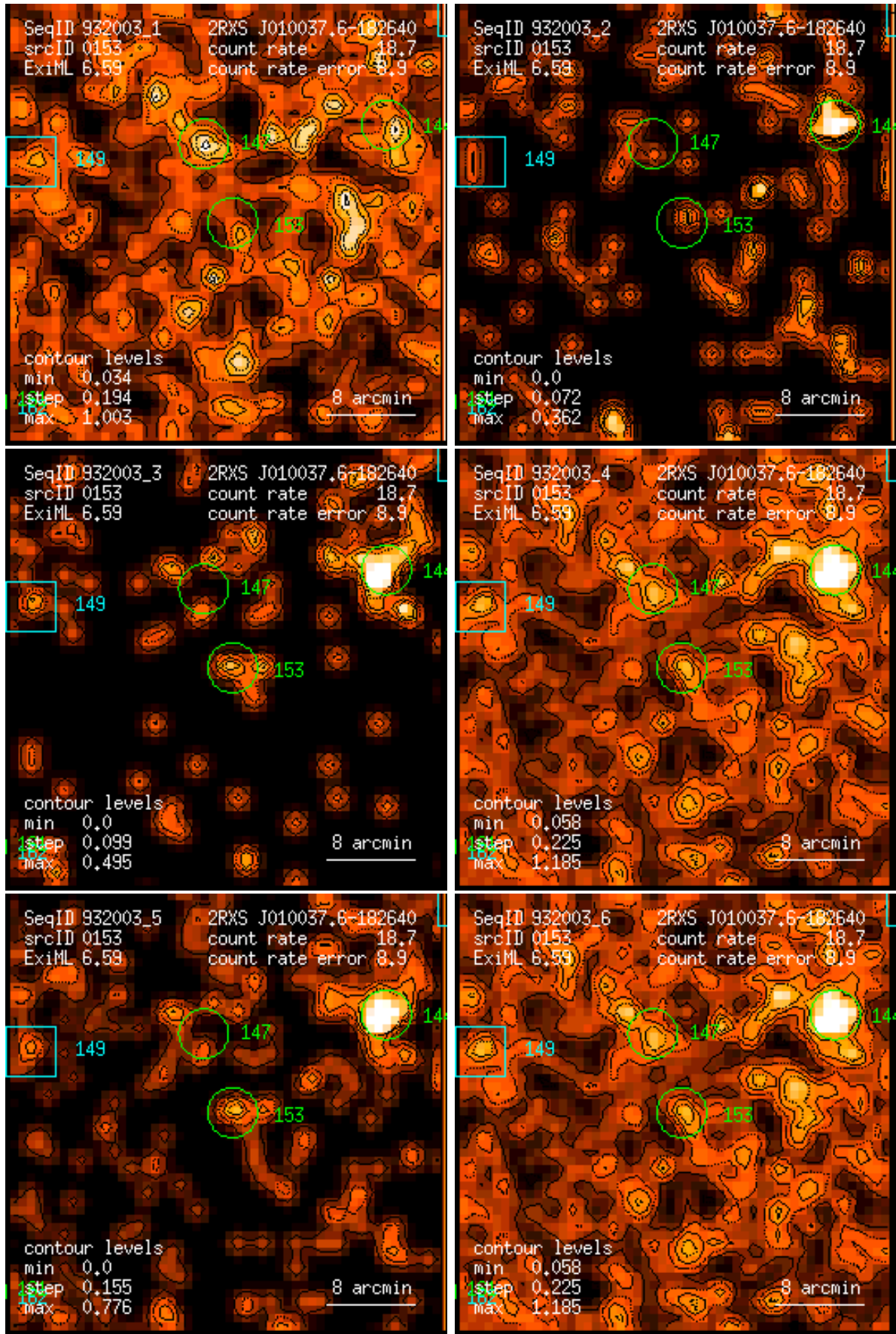
Figure 153: RASS 932003: detection 0153: band rate images, Gaussian filter: (1) PSPC channels 11 – 41, (2) 52 – 90, (3) 91 – 201, (4) 11 – 235, (5) 52 – 201, (6) 11 – 201. Broad band rates in counts/ks. Band rate contour levels in counts/ks/arcmin 2 .
