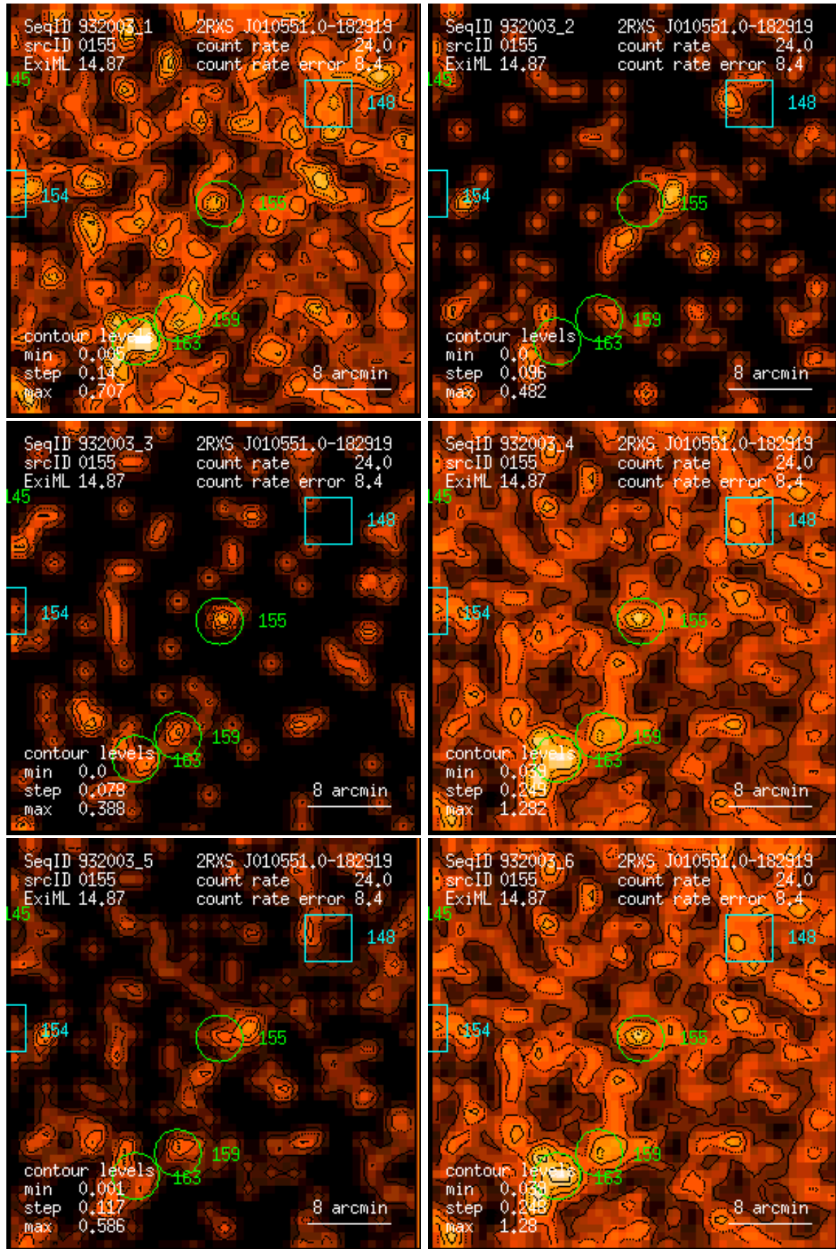
Figure 155: RASS 932003: detection 0155: band rate images, Gaussian filter: (1) PSPC channels 11 – 41, (2) 52 – 90, (3) 91 – 201, (4) 11 – 235, (5) 52 – 201, (6) 11 – 201. Broad band rates in counts/ks. Band rate contour levels in counts/ks/arcmin 2 .
