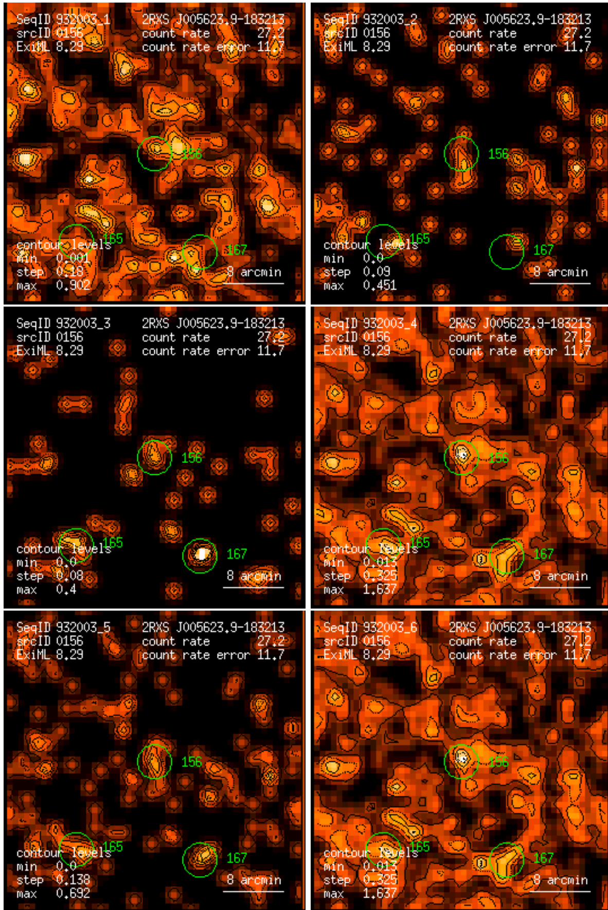
Figure 156: RASS 932003: detection 0156: band rate images, Gaussian filter: (1) PSPC channels 11 – 41, (2) 52 – 90, (3) 91 – 201, (4) 11 – 235, (5) 52 – 201, (6) 11 – 201. Broad band rates in counts/ks. Band rate contour levels in counts/ks/arcmin 2 .
